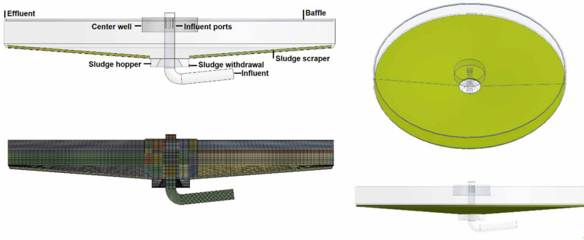
Figure 1 | 3D geometry and the mesh of original circular PST.
