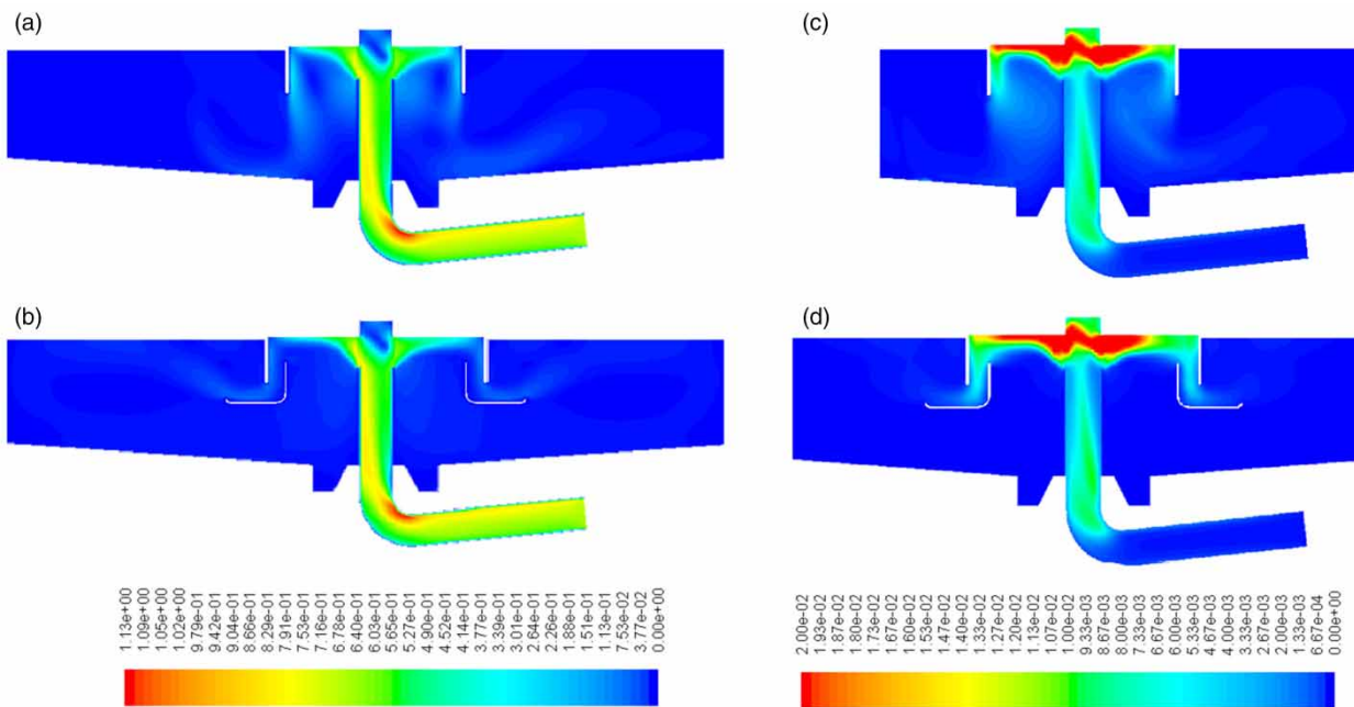
Figure 6 | Velocity contours (m/s) (a) OPST and (b) NPST and contour of turbulence kinetic energy (m 2 /s 2 ) (c) OPST and (d) NPST.
