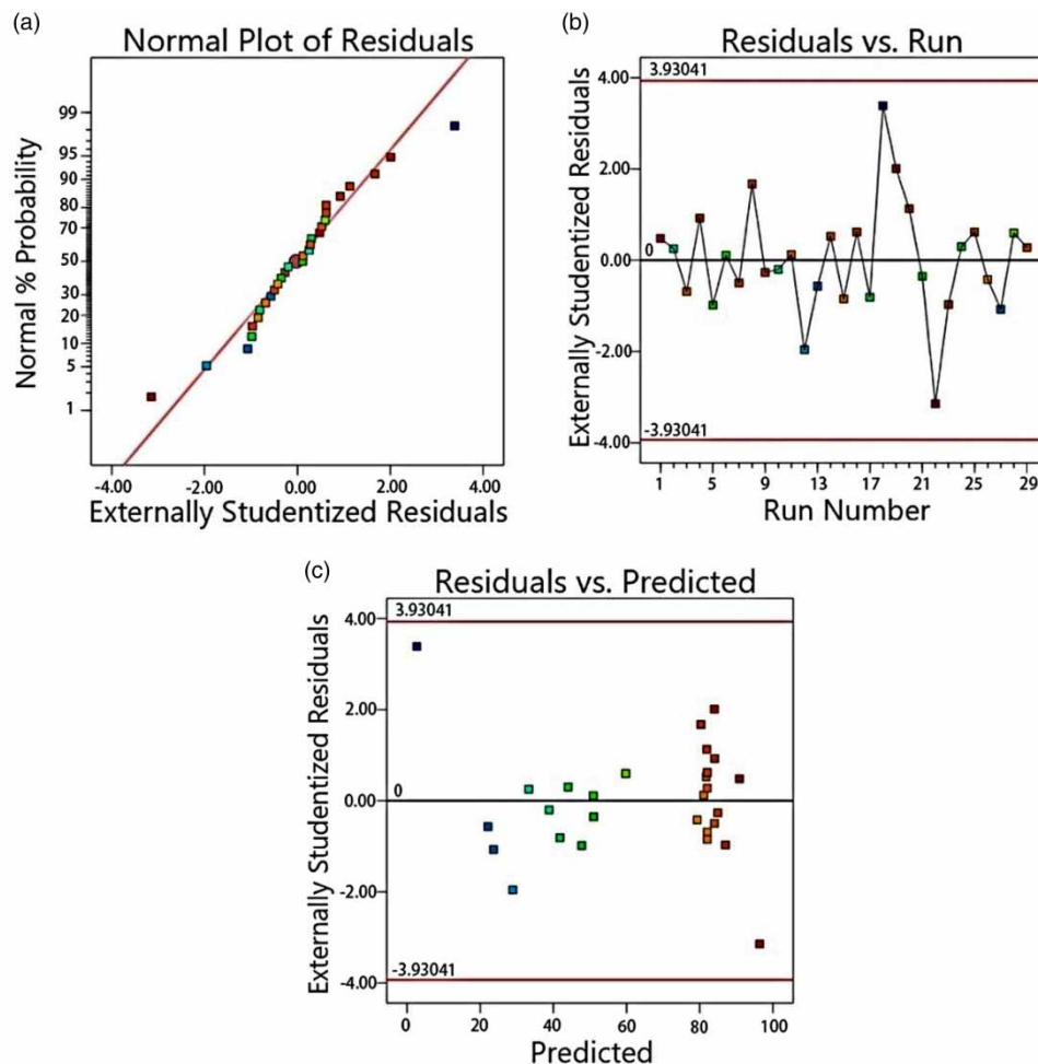
Figure 5 | Residual plots of Cr(VI) removal efficiency using S-nZVI@H, (a) residuals normal possibility diagram, (b) the chronological diagram of residuals, (c) residuals graph based on predicted values.
