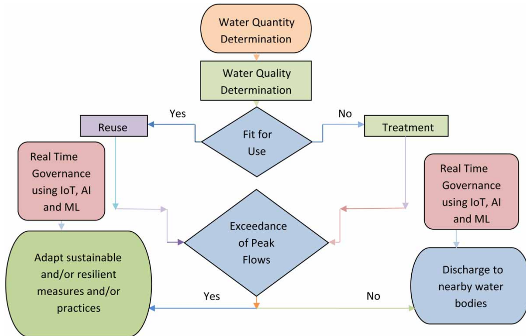
Figure 2 | Process diagram of integrated urban stormwater management.
