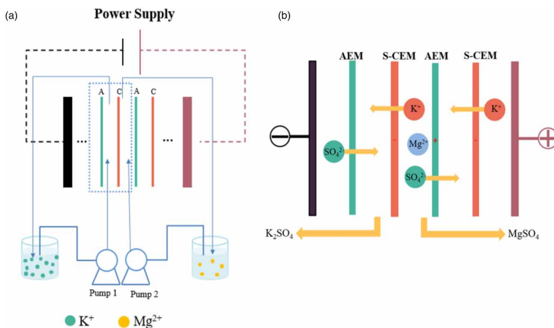
Figure 1 | Schematic diagrams of the experimental device and process: (a) experimental device of SED and (b) principle of ion migration mechanism.
