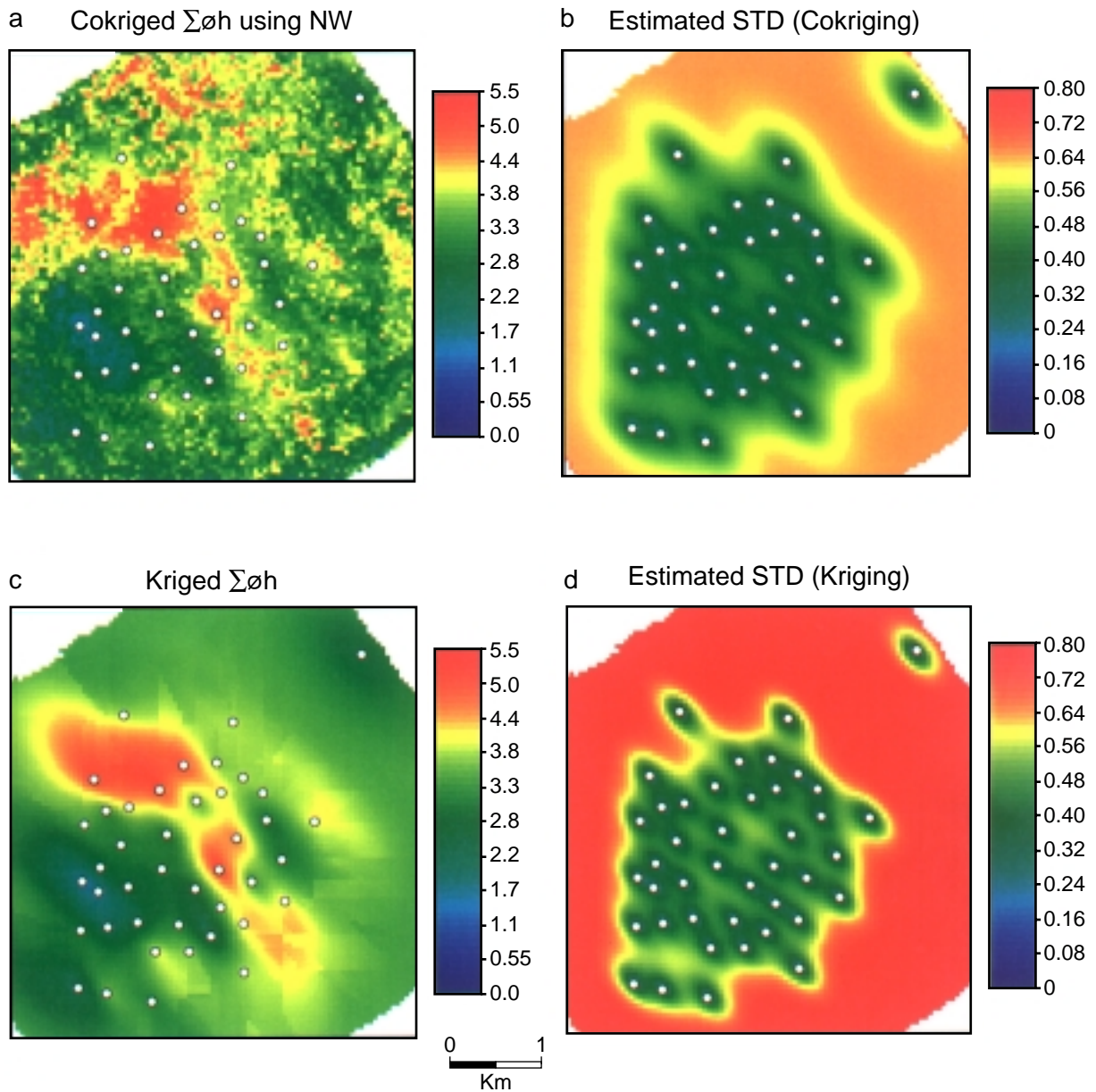
Figure 6: (a) Cokriged \Sigma\emptyset h distribution. (b) The estimated standard deviation by cokriging. (c) Kriged \Sigma\emptyset h distribution. (d) The standard deviation by kriging. White small circles in each figures indicate the well locations across the reservoir unit.
