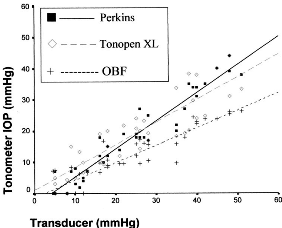
FIGURE 5. Scatterplot of actual IOP (transducer measured) against IOP estimates measured by tonometers. Lines: univariate regression summarizing the relationship between the two variables.
