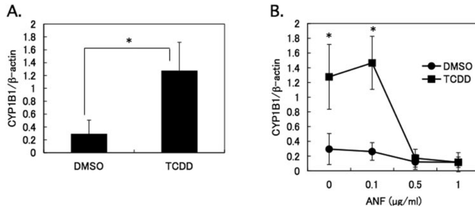
FIGURE 4. CYP1B1 expression in human retinal pigment epithelial cells cultured with TCDD. (A) CYP1B1 mRNA expression in ARPE-19 cells cultured with 1 nM TCDD or DMSO alone was analyzed by real-time PCR. TCDD treatment increased CYP1B1 mRNA expression in ARPE-19 cells. (B) ARPE-19 cells were cultured with 1 nM TCDD (closed squares) or DMSO alone (closed circles) in the presence of the indicated concentrations of ANF, and CYP1B1 mRNA expression was measured. Higher concentrations of ANF strikingly inhibited TCDD-stimulated CYP1B1 mRNA expression in ARPE-19 cells. Data are presented in mean \pm SEM of triplicate assays. *Significant difference ( P < 0.05 ). Experiments were repeated three times with similar results.
