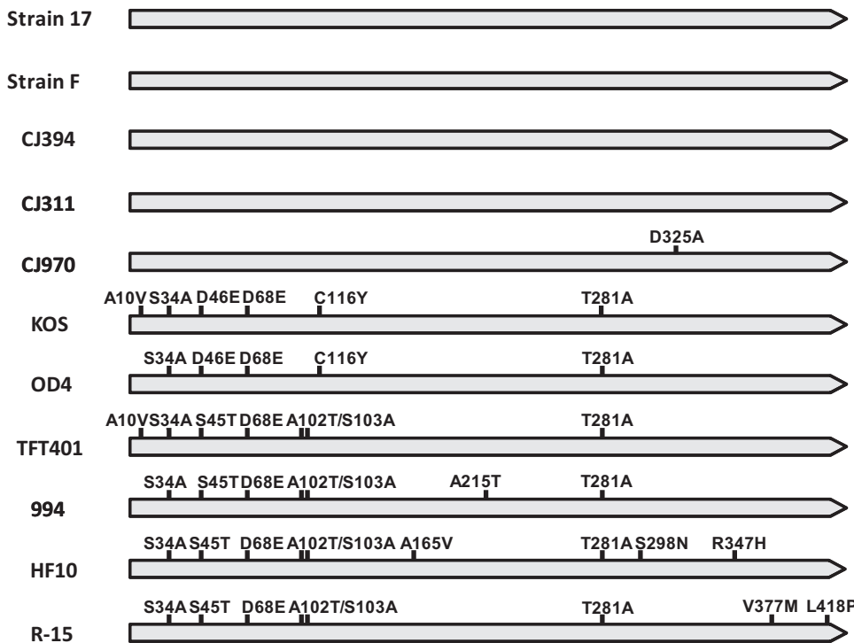
FIGURE 1. Sequence variability in the HSV-1 U s 1 ( \alpha 22) protein. Filled arrows : U s 1 protein for each strain of virus, with amino acid differences indicated by vertical bars with the sequence differences noted. Only the amino acids different from the strain 17 sequence are shown.
