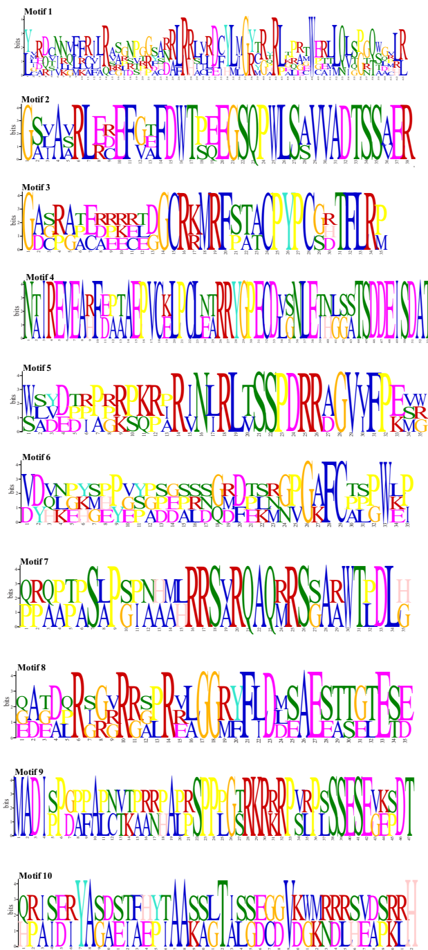
FIGURE 4. MEME analysis for conserved motifs within the \alpha -herpesvirus \alpha 22 protein. Motif detection was limited to a phylogenetically relevant n = 10 . The sequence of each of the motifs is presented; the larger the letter, the greater the conservation.
