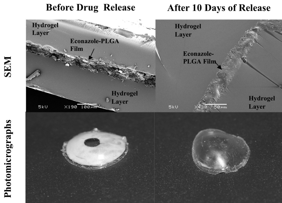
FIGURE 4. Scanning electron and photomicrographs of econazole-PLGA films within pHEMA hydrogels before and after 10 days of drug release. Magnification: top left , \times 190 ; top right , 430\times magnification.
