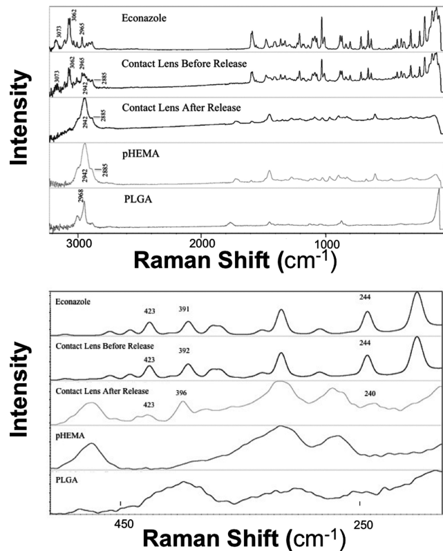
FIGURE 5. Raman spectra of econazole, a pHEMA film, a PLGA film, and a contact lens containing an econazole-PLGA film (PLGA 16 ) before and after 10 days of drug release. Top : shift from 0 to 3300 \text{ cm}^{-1} . Zoom of the Raman spectra ( bottom , 180\text{--}550 \text{ cm}^{-1} ) demonstrated multiple peaks ( 423, 391, \text{ and } 244 \text{ cm}^{-1} ) in the contact lens that were indicative of econazole.
