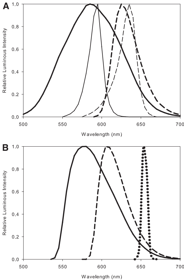
FIGURE 1. Normalized spectral luminous intensities of red and yellow signals in (A) railway signals measured in the laboratory: yellow incandescent ( thick solid line ), yellow LED ( fine solid line ), red incandescent ( thick dashed line ), and red LED ( fine dashed line ) and in (B) experiment 1: yellow signal ( solid line ), red signal ( dashed line ) and narrow-band red signal ( dotted line ). The CIE chromaticity coordinates of the railway signals are yellow incandescent (0.57, 0.43), yellow LED (0.58, 0.42), red incandescent (0.72, 0.28), and red LED (0.71, 0.29). The CIE chromaticity coordinates of the signals in experiment 1 are given in the Methods section.
