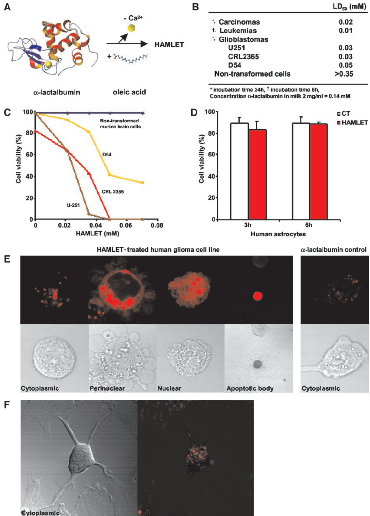
Fig. 1. HAMLET structure and function in vitro . A , HAMLET is formed from native \alpha -lactalbumin by removal of \text{Ca}^{2+} and by addition of the C18:1, 9 cis fatty acid (13). The figure is based on the \alpha -lactalbumin crystal structure (33). B , sensitivity of tumor cell lines to HAMLET. LD 50 , concentration required to kill 50% of the cells in 6/24 h. C , dose response of glioma cell lines to HAMLET. Murine primary brain cell cultures were used as controls. D , resistance of nontransformed human astrocytes to HAMLET treatment (0.03 mM). E , cellular trafficking of HAMLET in malignant glioma cells. HAMLET (red, top panels) binds to the tumor cell surface, invades their cytoplasm, translocates to the perinuclear region, and accumulates in the nuclei. Morphological changes include membrane blebbing, nuclear condensation, vesicle formation, cell shrinkage, and formation of apoptotic bodies (light transmission; bottom panels, magnification, \times 180 ). \alpha -Lactalbumin binds to the surface and enters the cytoplasm in small amounts but does not relocate to the nucleus. Trypan blue marks dead cells. F , localization of HAMLET in nontransformed human astrocytes. HAMLET enters the cytoplasm, forming small aggregates, but does not relocate to the cytoplasm. The cells remain viable for at least 24 h.
