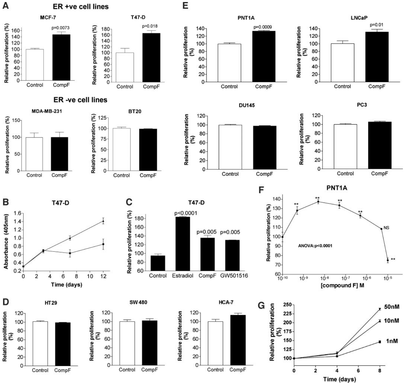
Fig. 2. Activation of peroxisome proliferator-activated receptor \delta (PPAR \delta ) stimulates proliferation of a subset of epithelial cell lines. A , effect of compound F on cell proliferation in breast cancer cells. The figure shows growth stimulation of estrogen receptor-positive (ER +ve) breast cancer cells by compound F (CompF). Human breast cancer cells were grown in phenol red-free medium with 5% dextran charcoal-stripped FCS (DCFCs) and were treated with 10 nM compound F; relative cell numbers were determined at day 12. Relative proliferation at the final time point are expressed in percentage control \pm SE ( n = 3-6 ); ER -ve, estrogen receptor negative. B , shown is a time course of T47D cells growing with (triangles) and without (squares) 10 nM compound F. C , shown is the relative stimulation of proliferation of T47D cells by estradiol compared with compound F (CompF; 10 nM) and an additional PPAR \delta agonist, GW501516 (20 nM) for 14 days. D , effect of compound F (CompF; 10 nM) on cell proliferation in human colon cancer cell lines. Relative proliferation at day 12 is shown. E , effect of compound F (CompF; 10 nM) on proliferation in prostate cell lines. The figure shows that compound F stimulates proliferation in androgen-sensitive PNT1A and LNCaP cells, but not in androgen-insensitive DU145 and PC3 cells. Relative proliferation at day 12 is shown. F , a dose response to compound F treatment of PNT1A cells for 6 days is shown with the maximum growth stimulation being observed at 10 nM. **, P < 0.001 , in a Dunnett's post-test relative to the control cultures. G , an additional PPAR \delta ligand, GW501516, also stimulates the proliferation of PNT1A cells in a dose- and time-responsive fashion. The proliferation of the drug-treated cultures is expressed as a percentage of the value obtained with the control cultures. Error bars, SE from three triplicate cultures. Each experiment was repeated three times.
