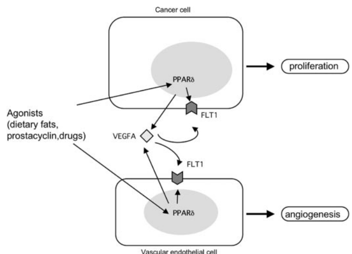
Fig. 9. A proposed model of the action of peroxisome proliferator-activated receptor \delta (PPAR \delta ) in tumor growth and angiogenesis. Activation of PPAR \delta is associated with increased expression of vascular endothelial growth factor \alpha (VEGF \alpha ) and FLT-1. Locally produced VEGF \alpha can result in the activation of FLT-1 receptor. PPAR \delta may also have paracrine effects whereby VEGF \alpha that is produced in the cancer cells can bind to FLT1 and FLT-1 receptors expressed on endothelial cells. This effect may be further augmented by the PPAR \delta -mediated up-regulation of FLT-1 in endothelial cells.
