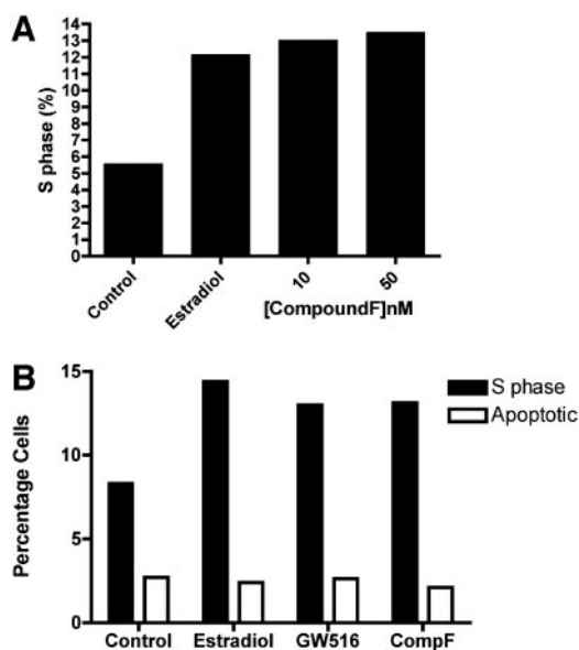
Fig. 6. Compound F and GW501516 increase the number of cells in active cell division. A, T47D cells were grown in 5% dextran charcoal-stripped FCS with solvent alone (Control), or estradiol (Estradiol, 10 nM), or compound F (CompoundF, 10 nM) for 7 days. The cells were then labeled with bromodeoxyuridine and propidium iodide and were subjected to fluorometric cell-sorting analysis. The percentage of cells in S phase is shown. B, T47D cells were grown in 0.1% FCS with solvent alone (Control), estradiol (Estradiol, 10 nM), GW501516 (GW516, 25 nM), or compound F (CompF, 10 nM). Black bars, the percentage of cells in S phase; white bars, the percentage of cells in apoptosis.
