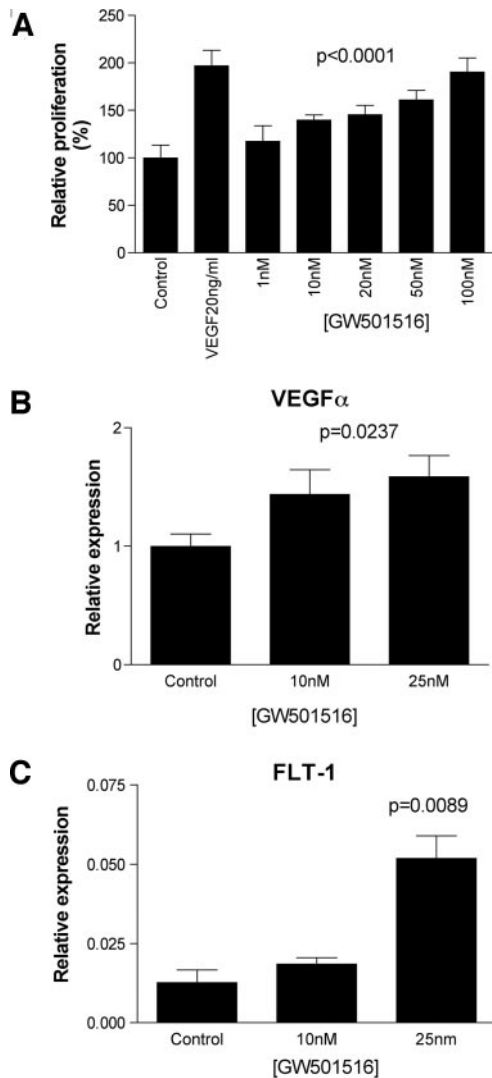
Fig. 8. GW501516 stimulates proliferation of human umbilical vein endothelial cells (HUVECs). A , HUVECs were treated with vehicle (Control), 20 ng/ml human recombinant vascular endothelial growth factor (VEGF) \alpha -165 (VEGF \alpha ) or 1, 10, 20, 50, and 100 nM GW501516 for up to 14 days. Shown is the relative proliferation. B , peroxisome proliferator-activated receptor \delta (PPAR \delta ) activation is associated with increased expression of VEGF \alpha mRNA. Shown here is the relative mRNA levels of VEGF \alpha in response to treatment of HUVECs with 0, 10, and 25 nM GW501516 for 22 h. C , PPAR \delta activation is associated with increased expression of FLT-1 mRNA. Shown is the relative mRNA levels of FLT-1 in response to treatment of HUVEC with 0, 10 and 25 nM GW501516 for 22 h. The dose response was analyzed using one-way ANOVA, with a post-test for trend. The P is shown for the post test. The error bars represent SE of three triplicate cultures. Each experiment was performed twice.
