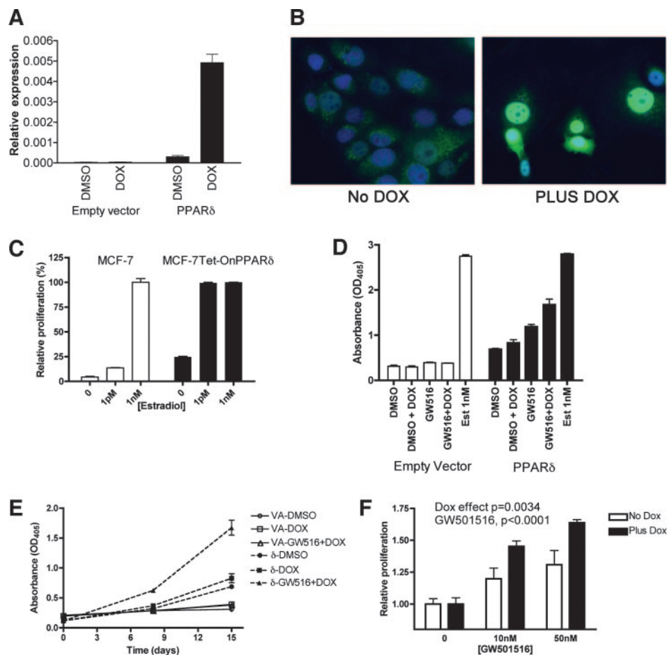
Fig. 7. Doxycycline (DOX)-regulated peroxisome proliferator-activated receptor \delta (PPAR \delta ) expression increases the proliferative response to GW501516. MCF7 Tet-On human PPAR \delta (hPPAR \delta ) and MCF7 Tet-On empty vector cells were treated with 2 \mu g/ml DOX (PLUS DOX) or solvent alone (No DOX) for 48 h. A, the steady-state levels of mRNA encoding PPAR \delta were measured by quantitative real-time-PCR. B, PPAR \delta protein levels were visualized by fluorescence-based immunohistochemistry. PPAR \delta was visualized using FITC (green), and the chromatin was counterstained with 4',6-diamidino-2-phenylindole (blue). C, MCF7 and MCF7 Tet-On hPPAR \delta cells were cultured with different concentrations of estradiol. D, MCF7 Tet-On hPPAR \delta cells and MCF7 Tet-On empty vector cells were grown for 15 days in the presence or absence of DOX and/or GW501516 (GW516, 50 nM). The relative cell proliferation was determined. Est, estradiol. E, the time dependency of this experiment is shown. VA-DMSO, vector alone + vehicle; VA-DOX, vector alone + DOX; VA-GW516+DOX, vector alone +GW501516+DOX; \delta -DMSO, PPAR \delta +vehicle; \delta -DOX, PPAR \delta +DOX; \delta -GW516+DOX, PPAR \delta +GW501516+DOX. F, the effects of GW501516 and DOX were tested by two-way ANOVA, and the resulting P s are shown. Error bars, the SE of three replicate cultures. The experiment was repeated four times.
