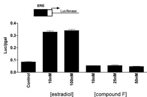
Fig. 4. Compound F cannot activate an estrogen response element (ERE). The pERE-Luc reporter plasmid was transfected into T47D cells, and the cells were assessed for a response to 10 nM compound F. Error bars, the SE of three replicate cultures. This experiment was performed twice.
