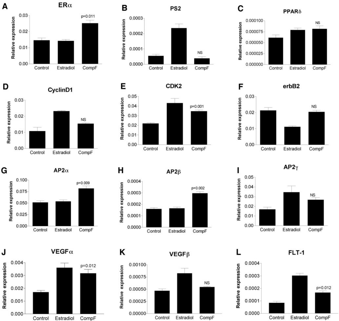
Fig. 5. Compound F modulates distinct growth regulation genes compared with estrogen. T47D cells were treated with DMSO ( Control ), 10 nM estradiol ( Estradiol ), or 10 nM compound F ( CompF ) for 22 h, and RNA was prepared from the cells. The expression of putative target genes was measured using quantitative real-time PCR. Error bars, SE of three replicate cultures. The experiment was repeated three times. ER, estrogen receptor; PPAR, peroxisome proliferator-activated receptor; VEGF, vascular endothelial growth factor.
