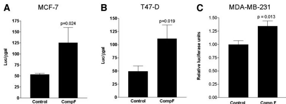
Fig. 3. Effect of compound F on peroxisome proliferator response element driven luciferase reporter in human breast cancer cells. The pFAB-PLuc reporter construct was transfected into T47D (A), MCF7 (B); and MDAMB-231 (C) cells and was assessed for a response to 10 nM compound F (CompF). Error bars, the SE of 3–6 replicate cultures, and each experiment was repeated twice or more. The results shown for MDA-MB-231 (C) are pooled from three separate experiments to test the significance of the marginal induction observed.
