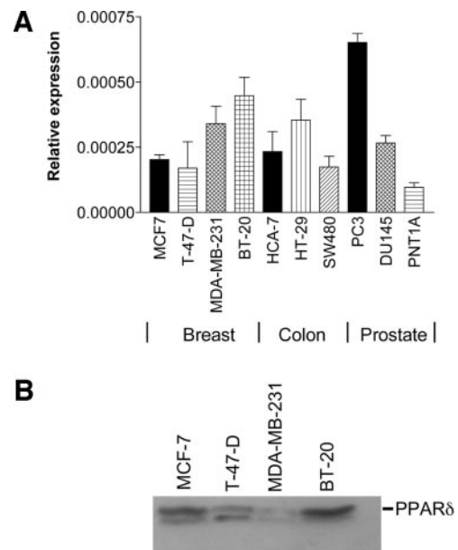
Fig. 1. Peroxisome proliferator-activated receptor \delta (PPAR \delta ) expression in breast, colon, and prostate cancer cell lines. A , the steady-state levels of mRNA encoding PPAR \delta in a panel of human epithelial cancer cell lines was quantified by quantitative real-time PCR and normalized to 18S rRNA levels. B , PPAR \delta protein levels in human breast cancer cells were determined by Western blotting using a polyclonal antiserum raised against the full-length human PPAR \delta . Shown are the signals obtained with MCF7, T47D, MDA-MB-231, and BT-20 cells. Protein levels do not correlate well with mRNA levels, because MDA-MB-231 have consistently lower levels of PPAR \delta protein compared with the other cell lines; however they express similar amounts of PPAR \delta mRNA. Shown is a representative blot of three independent experiments.
