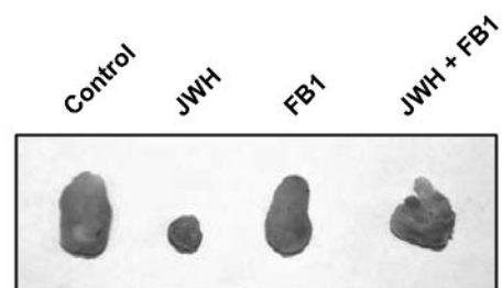
Fig. 5. Changes in the size of mouse gliomas after cannabinoid and fumonisin B1 treatment. Animals bearing gliomas ( n = 4-6 for each experimental group) were treated with either vehicle ( Control , ○), JWH-133 ( JWH , ●), fumonisin B1 ( FB1 , □), or JWH-133 plus fumonisin B1 (■) for up to 8 days as described in "Materials and Methods." Examples of formaldehyde-fixed dissected tumors after 8 days of treatment are shown. Bars, \pm SD.
