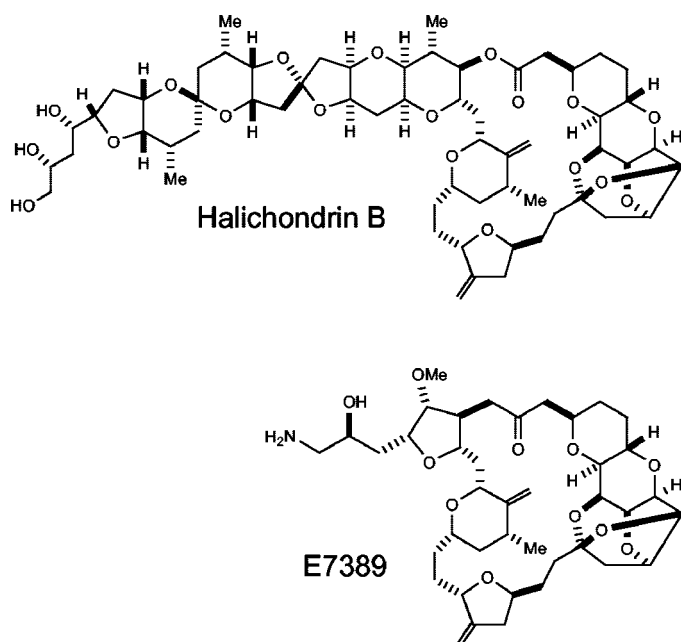
Fig. 1. Structures of halichondrin B and E7389
