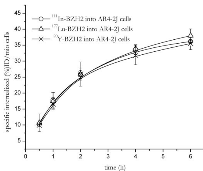
Fig. 6. Comparison of the internalization rate of [ ^{111}\text{In} ]-BZH2 (○), [ ^{90}\text{Y} ]-BZH2 (×) and [ ^{177}\text{Lu} ]-BZH2 (△) into AR4-2J cells. Data result from two independent experiments with triplicates in each experiment and are expressed as specific internalization; bars, \pm SD.
