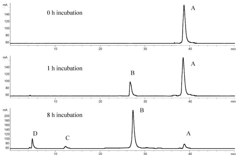
Fig. 2. HPLC elution profile of [ ^{111}\text{In} ]-BZH1 after incubation with fresh human serum, immediately after incubation, t_R = 38.7 min; 1 hour after incubation, t_R ([ ^{111}\text{In} ]-BZH1) = 38.6 minutes, t_R (metabolite B) = 27.3 min; 8 hours after incubation, t_R ([ ^{111}\text{In} ]-BZH1) = 38.7 minutes, t_R (metabolite B) = 27.5 minutes, t_R (metabolite C) = 12.3 minutes, t_R (metabolite D) = 5.1 minutes.
