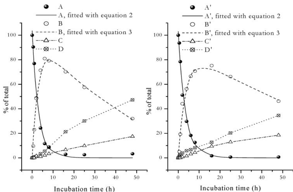
Fig. 3. Comparison of kinetic stability of [ ^{111}\text{In} ]-BZH1 (left) and [ ^{111}\text{In} ]-BZH2 (right) in fresh human serum. Percentage of total peptide after different incubation times with serum under 37°C, 5% \text{CO}_2 , the concentration is 0.6 nmol radiolabeled peptide per mL serum.
