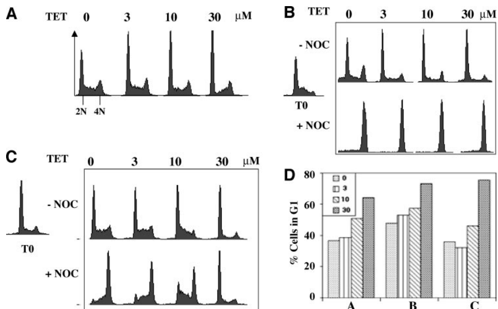
Fig. 3. Tetrandrine induces early G 1 -phase arrest. A , Exponentially growing HT29 cells were treated with the indicated concentrations of tetrandrine for 18 hours. B , HT29 cells were first synchronized in early S phase with 1 \mu\text{mol/L} aphidicolin for 24 hours (T0). After aphidicolin removal (by rinsing the cultures in drug-free medium) and further incubation in fresh medium for 1 hour, cultures were further incubated in the presence of the indicated tetrandrine concentrations alone or tetrandrine plus nocodazole (0.2 \mu\text{g/mL} ) for 18 hours. C , HT29 cells were first synchronized in G 0 in medium containing 0.04% FBS for 24 hours. Cells then were incubated in normal medium containing 10% FBS in the presence of tetrandrine alone or tetrandrine plus nocodazole for 15 hours. D , quantification of the G 1 -phase population corresponding to protocols A, B, and C. The DNA content distribution histograms of fluorescence-activated cell-sorting analysis were measured by flow cytometry. The different phases of the cell cycle were determined with ModFit DNA analysis software. Data shown are representative of at least three independent experiments.
