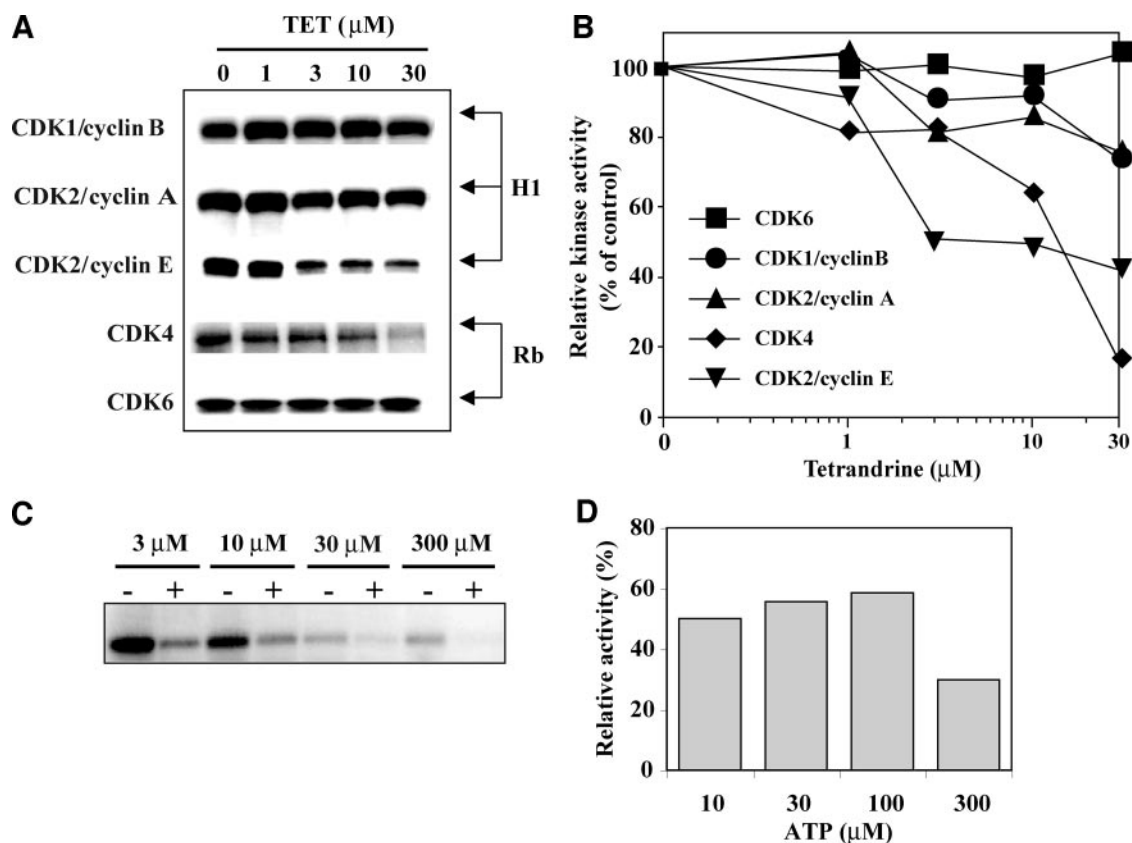
Fig. 6. Effect of tetrandrine on the activities of CDKs in vitro . A , Purified CDK1/cyclin B, CDK2/cyclin A, CDK2/cyclin E, or CDK6/cyclin D3 active complexes were incubated with [ \gamma - ^{32} P]ATP, histone H1, and the indicated concentrations of tetrandrine for 30 minutes at 30°C. CDK4 immune complexes were prepared from exponentially growing HT29 cells and reacted with [ \gamma - ^{32} P]ATP, a Rb polypeptide, and tetrandrine for 30 minutes at 30°C. B , quantification of the inhibitory activity of tetrandrine from the data shown in A using ImageQuant software (Molecular Dynamics). Data shown are representative of at least two independent experiments. C , effect of ATP on inhibition of CDK4 by tetrandrine. CDK4 immunoprecipitation kinase assays were performed in the presence of the indicated ATP concentrations. D , quantification of relative CDK4 activity in the presence of tetrandrine and increasing ATP concentration.
