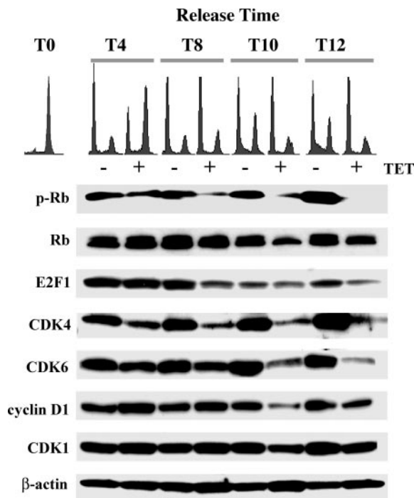
Fig. 7. Effect of tetrandrine on Rb phosphorylation and levels of cyclin D1 and CDKs in HT29 cells following synchronization in G 2 -M phase with 0.2 \mu g/mL nocodazole for 15 hours (T0). Times after nocodazole release (by washing out nocodazole) and further incubation in fresh medium with or without tetrandrine are indicated at the top of the figure.
