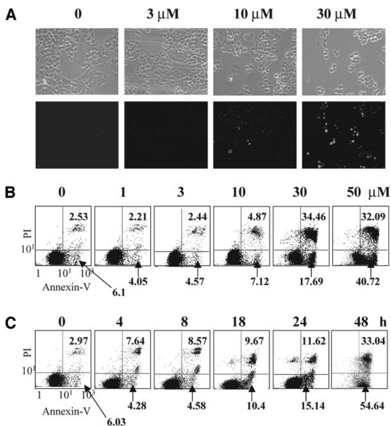
Fig. 5. Tetradrine-induced apoptosis in HT29 cells. A , detection of apoptosis by TUNEL assay. Cells were treated with the indicated concentrations of tetradrine for 24 hours (0, control untreated cells). Top , phase contrast microscopy; bottom , fluorescence detection. B and C , detection of apoptosis by annexin V and PI staining. B , Cells were treated with the indicated concentrations of tetradrine for 24 hours. C , time course in cells treated with 30 μmol/L tetradrine for 4, 8, 18, 24, and 48 hours, respectively. The percentage of annexin V-positive cells in the top (PI negative) and bottom (PI positive) right quadrants is indicated.
