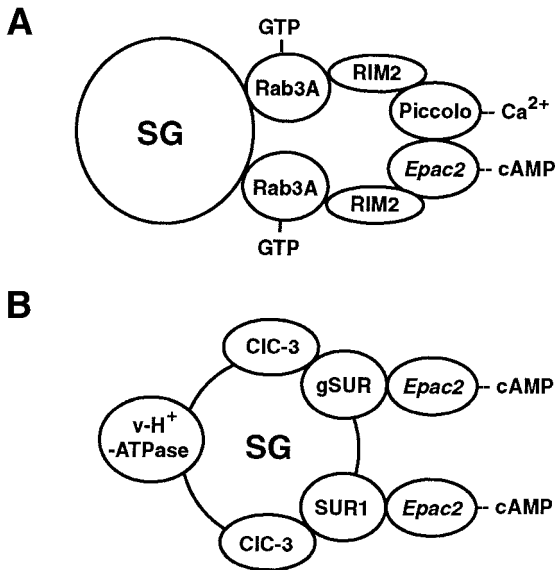
FIG. 3. Epac as a regulator of insulin granule exocytosis. A: Depicted are cAMP- and Ca 2+ -dependent interactions of Epac2 , Rim2, and Piccolo based on an as yet to be established stoichiometry of 1:2:1. The Epac2 -Rim2-Piccolo macromolecular complex interacts with the GTP-bound form of Rab3A to regulate the priming and exocytosis of secretory granules (SG) (5–7). B: Epac2 stimulates exocytosis by interacting with insulin granule-associated sulfonylurea receptors (gSUR and SUR1) that regulate the activity of CIC-3 channels. Uptake of Cl − into the granule facilitates granule acidification and priming mediated by the V-type H + -ATPase (11). Not illustrated are possible interactions of Epac2 with plasma membrane-associated SUR1.
