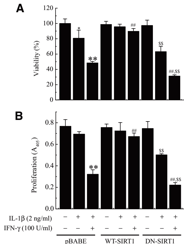
FIG. 3. Effects of SIRT1 overexpression on cytokine-induced cytotoxicity. Control or SIRT1-overexpressing RIN cells ( 1 \times 10^5 ) were treated with IL-1 \beta alone or IL-1 \beta and IFN- \gamma for 48 h. The cell viability (A) and cell proliferative potential (B) were then determined using an MTT and BrdU incorporation assay, respectively. Each value represents the mean \pm SE of three independent experiments. * P < 0.05 , ** P < 0.01 vs. untreated pBABLE; ## P < 0.01 vs. IL-1 \beta + IFN- \gamma -treated pBABLE; $$ P < 0.01 vs. untreated DN-SIRT1.
