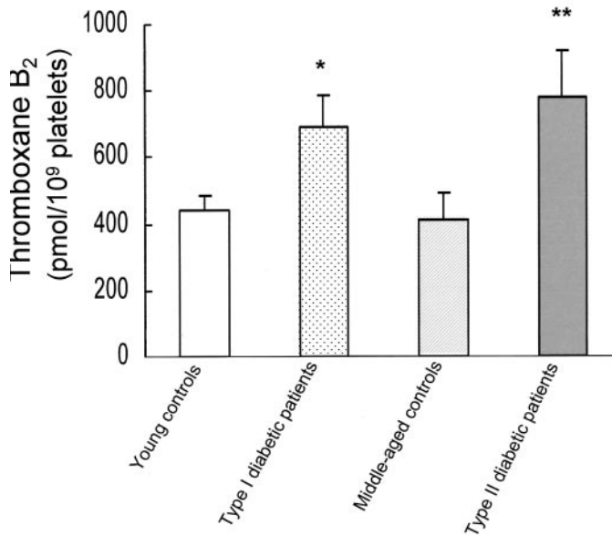
FIG. 1. Basal formation of TxB 2 in unstimulated platelets from both type 1 and type 2 diabetic patients and from respective control subjects. Results are expressed as the means ± SE ( n = 9). * P < 0.05; ** P < 0.03.
