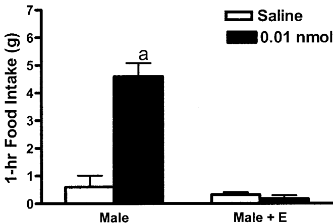
FIG. 3. i3vt ghrelin increases food intake in males but not in males administered estradiol. Control males (Male; n = 10 ) and males injected subcutaneously with 2 \mu\text{g} 17 \beta -estradiol benzoate (2 days earlier to mimic plasma estradiol levels of females in estrus) (Male + E; n = 10 ) were administered i3vt ghrelin (0.01 nmol/1 \mu\text{l} saline) and vehicle (1 \mu\text{l} saline) on separate days. Data are expressed as means \pm SEM percent of vehicle baseline. * P < 0.05 vs. vehicle.
