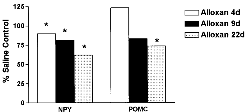
FIG. 4. ARC NPY and POMC mRNA expression 4, 9, and 22 days after 3v alloxan as a percent of their respective saline controls tested contemporaneously at each individual time point. * P \leq 0.05 vs. 3v saline-injected rats.
