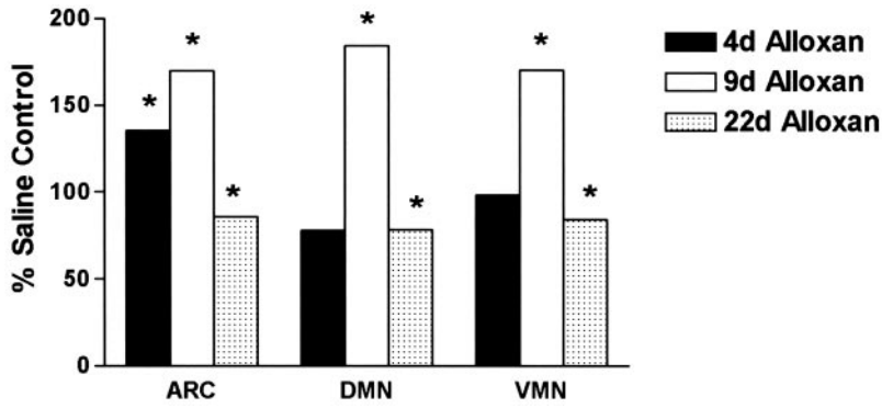
FIG. 3. GK mRNA expression in the VMN, DMN, and ARC hypothalamic nuclei 4, 9, and 22 days after 3v alloxan as a percent of their respective saline controls tested contemporaneously at each individual time point. * P \leq 0.001 vs. 3v saline-injected rats.
