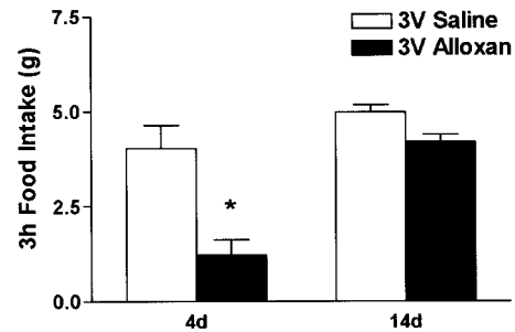
FIG. 1. Food intake (g) over 3 h after systemic 2DG (250 mg/kg, s.c.) administered to nonfasted rats 4 or 14 days after 3v alloxan or saline injection. Data are means \pm SEM. * P \leq 0.01 vs. 3v saline-injected rats tested at 4 days.
