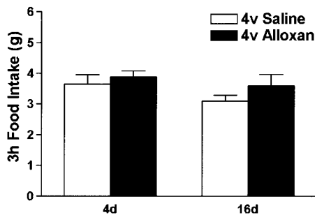
FIG. 6. Food intake in response to subcutaneous 2DG (250 mg/kg) administration 4 or 16 days following 4v alloxan or saline injection. 2DG injections were given immediately before presentation of food. Data are means \pm SEM.
