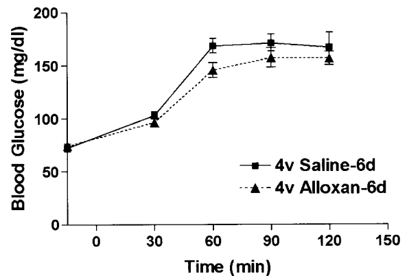
FIG. 7. Effect of systemic 2DG (250 mg/kg, s.c.) on blood glucose concentrations (mg/dl) 6 days following 4v alloxan or saline injection. The 2DG injections were given to rats without food 15 min after the first blood sample was collected. Data are means \pm SEM.
