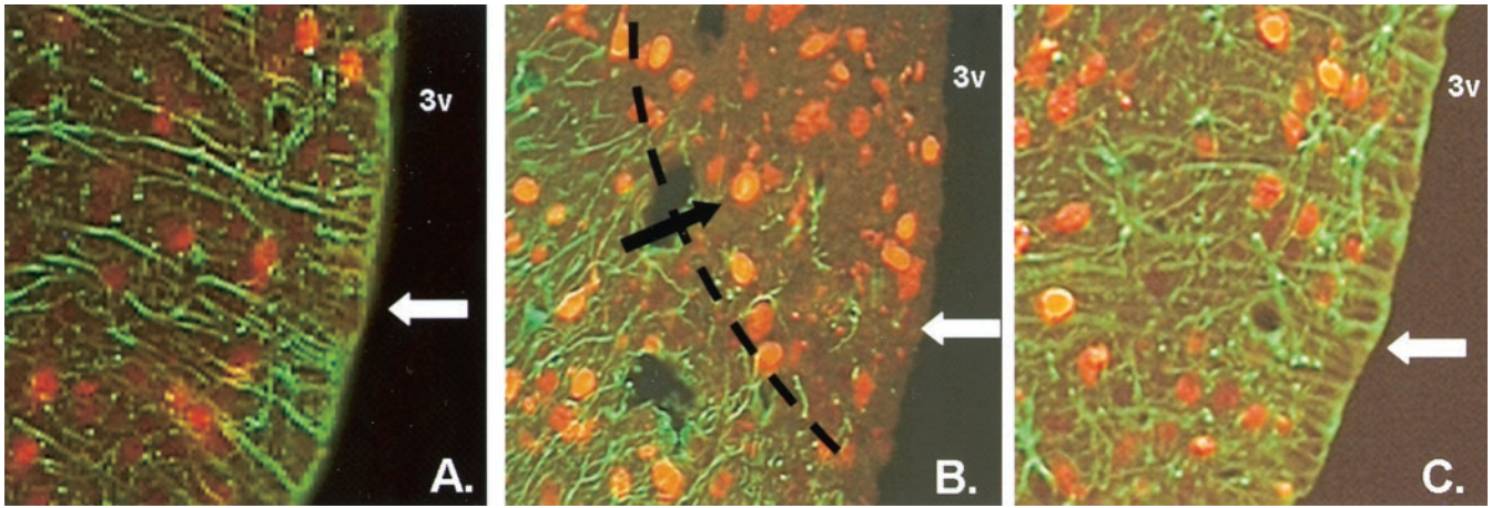
FIG. 5. Double-label immunohistochemistry for astrocytes (GFAP; green) and neurons (NeuN-ir; red) adjacent to the 3v and within the ventromedial hypothalamus in 3v saline-treated (A), 7-day post-3v alloxan-treated (B), and 14-day post-3v alloxan-treated (C) rats. Seven days following 3v alloxan injection, GFAP-ir cell bodies of \beta 1 and \alpha tanyctes lining the 3v wall were completely absent (white arrow, B) as compared with those in saline-treated rats (white arrow, A) and there was a circumscribed zone of absent GFAP-ir within the parenchyma surrounding the 3v (dashed line, B). Within this zone, NeuN-ir neurons appeared swollen (black arrow, B). By 14 days, GFAP-ir cell bodies lining the 3v and processes of \alpha and \beta 1 tanyctes extending into the parenchyma were restored (white arrow, C).
