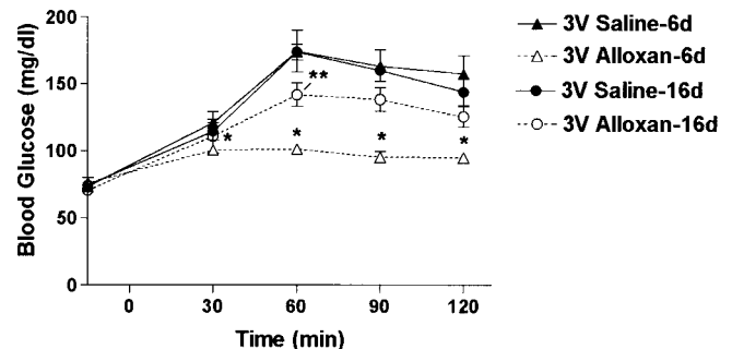
FIG. 2. Effect of systemic 2DG (250 mg/kg, s.c.) on blood glucose concentrations (mg/dl) 6 or 16 days following 3v alloxan or saline injection. The 2DG injections were administered to rats without food 15 min after the first blood sample was collected. Data are means \pm SEM. * P \leq 0.001 vs. 3v saline-injected rats tested at 6 days; ** P \leq 0.05 vs. 3v saline-injected rats tested at 16 days.
