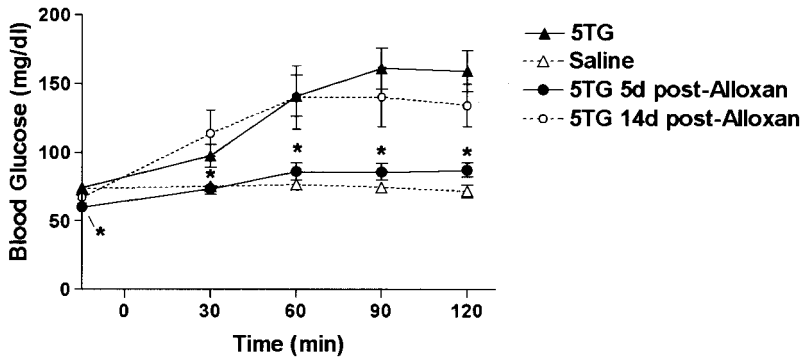
FIG. 8. Effect of 5TG (24 \mu g/200 nl) or saline injected into the caudal dorsomedial medulla on blood glucose concentrations (mg/dl) before and after 3v alloxan. Prior to 3v injections, saline or 5TG was injected into the dorsomedial medulla. 5TG-induced blood glucose responses were compared with blood glucose responses elicited by 5TG 5 days (5TG 5d post-Alloxan) and 14 days (5TG 14d post-Alloxan) after 3v alloxan. Data are means \pm SEM. * P \leq 0.05 vs. 5TG responses prior to 3v alloxan injection.
