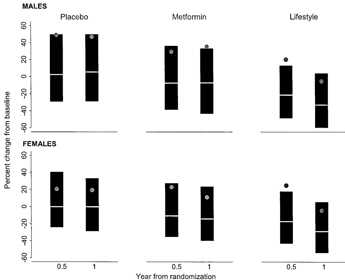
FIG. 1. Median percentage of change in CRP from baseline at month 6 and year 1 by sex. The data are presented as mean (gray dot), median (white line), and 25th (top of the gray box) and 75th percentiles (bottom of the gray box). At 6 months and at year 1 after randomization, the Wilcoxon's test yielded P < 0.001 for intensive lifestyle vs. metformin and intensive lifestyle vs. placebo in both men and women. After 6 months and 1 year of intervention, the P value from the Wilcoxon's test between metformin vs. placebo was <0.001 for women. Among men, the Wilcoxon's test for comparing metformin vs. placebo yielded P = 0.01 at 6 months and 0.006 at year 1.
