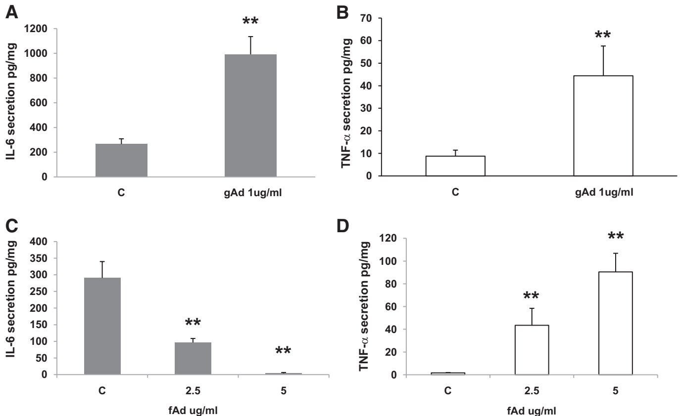
FIG. 4. A: IL-6 secretion was significantly (Student paired t test, P < 0.01 ) increased after incubation of cultured trophoblast cells with gAd (1 \mu g/ml). Data are mean \pm SEM for six placentas. B: TNF- \alpha secretion was significantly (Student paired t test, P < 0.01 ) increased after incubation of cultured trophoblast cells with gAd (1 \mu g/ml). Data are mean \pm SEM for six placentas. C: IL-6 secretion was significantly (RMANOVA, P < 0.01 ) reduced in a dose-dependent manner after incubation of cultured trophoblast cells with fAd (1 \mu g/ml). Data are mean \pm SEM for six placentas. D: TNF- \alpha secretion was significantly (RMANOVA, P < 0.01 ) increased in a dose-dependent manner after incubation of cultured trophoblast cells with fAd. Data are mean \pm SEM for six placentas. ** P < 0.01 .
