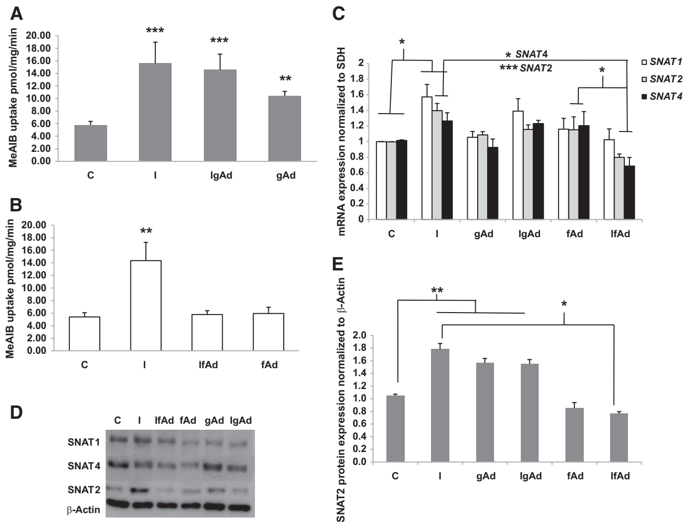
FIG. 2. Sodium-dependent ^{14}\text{C} -MeAIB uptake after incubation of cultured trophoblast cells in control media, insulin (1 nmol/l), gAd (5 \mu\text{g}/\text{ml} ) (A), or fAd (5 \mu\text{g}/\text{ml} ) (B) for 24 h. Subsets of cells were pretreated with insulin (1 nmol/l) for 4 h and then exposed to 5 \mu\text{g}/\text{ml} gAd (IgAd) or fAd (IfAd) for an additional 20 h. Data are mean \pm SEM for cells isolated from six different placentas. Insulin alone, gAd alone, and insulin + gAd ( P < 0.01 ) significantly stimulated MeAIB uptake; however, insulin + fAd significantly ( P < 0.001 ) reduced MeAIB uptake compared with insulin alone (RMANOVA with post hoc tests, *P < 0.05 , **P < 0.01 ). C: Summary data of real-time PCR of system A amino acid transporter isoforms SNAT1 , SNAT2 , and SNAT4 after incubation of cultured trophoblast cells as indicated. Data are mean \pm SEM for six placentas. Insulin significantly increased SNAT gene expression. In the presence of fAd, the effect of insulin on the mRNA expression of SNAT2 and SNAT4 was significantly reduced compared with both fAd and insulin treatment alone (RMANOVA, P < 0.01 ; Tukey-Kramer multiple comparisons post tests, *P < 0.05 , ***P < 0.01 ). D: Representative Western blot of SNAT1 , SNAT2 , and SNAT4 expression after incubation of cultured trophoblast cells as indicated. E: Summary of SNAT2 protein expression levels. n = 6 for each treatment, RMANOVA, P < 0.01 ; Tukey-Kramer multiple comparisons post tests, *P < 0.05 , **P < 0.01 .
