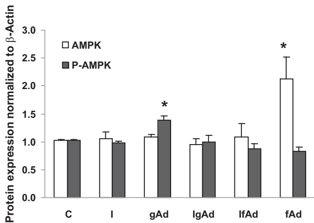
FIG. 3. Summary of phospho-AMPK and AMPK protein expression after incubation of cultured trophoblast cells with control media, insulin (1 nmol/l), gAd (5 \mu g/ml), or fAd (5 \mu g/ml) for 24 h. Subsets of cells were pretreated with insulin (1 nmol/l) for 4 h and then exposed to 5 \mu g/ml gAd (IgAd) or fAd (IfAd) for an additional 20 h. n = 5 placentas for each treatment. Phospho-AMPK expression was significantly increased by gAd (RMANOVA, P < 0.01 ). AMPK expression was significantly increased by fAd (RMANOVA, P < 0.002 ). Tukey-Kramer multiple comparisons post tests, * P < 0.05 .
