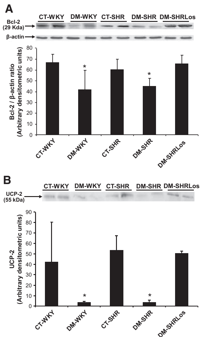
FIG. 7. A: Western blot analysis of Bcl-2 in total retinal lysate of the studied groups; the bars represent the means \pm SD of band densities expressed in arbitrary densitometric units from at least three independent experiments. * P < 0.05 . B: Western blot analysis of UCP-2 in immunoprecipitated retinal protein of the studied groups. The bars represent the means \pm SD of band densities expressed in arbitrary densitometric units from at least three independent experiments. * P = 0.03 . CT, control; DM, diabetic; Los, losartan.
