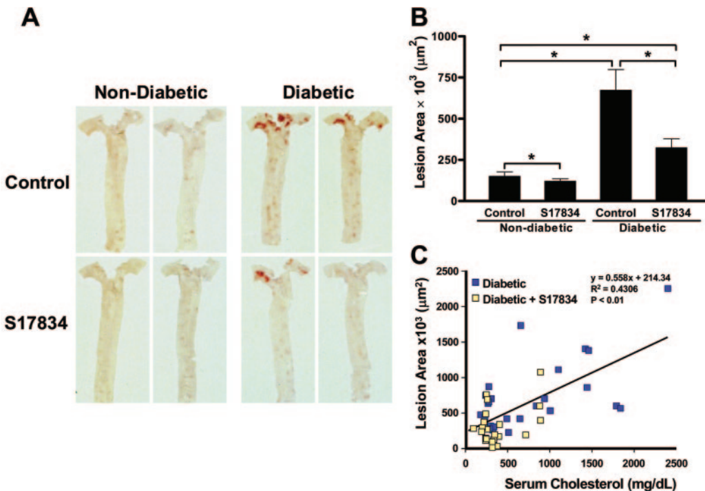
FIG. 8. Treatment with S17834 reduces aortic atherosclerotic lesions of STZ-induced diabetic LDLR ^{-/-} mice in large part through its lipid-lowering effect. A: S17834 attenuates aortic atherosclerotic lesions in diabetic LDLR ^{-/-} mice. A representative oil red O staining of aortic intima is shown in nondiabetic and diabetic LDLR ^{-/-} mice treated or not treated with S17834 ( 130 \text{ mg} \cdot \text{kg}^{-1} \cdot \text{day}^{-1} for 6 weeks). B: Quantitative analysis of oil red O-stained atherosclerotic lesions was performed using computer-assisted image analysis. Bar graph represents the means \pm SE ( n = 10-16 ). * P < 0.05 as indicated. C: Serum cholesterol concentrations were significantly correlated with aortic atherosclerotic lesion area in individual diabetic LDLR ^{-/-} mice treated or not treated with S17834.
