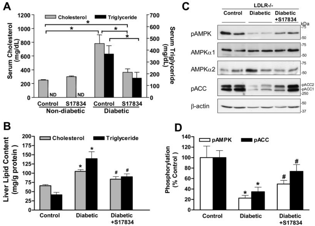
FIG. 7. Treatment with S17834 lowers serum and hepatic lipid levels as well as stimulates the phosphorylation of AMPK and ACC in the liver of STZ-induced diabetic LDLR ^{-/-} mice. A: S17834 reduces serum total cholesterol and triglyceride levels in diabetic LDLR ^{-/-} mice. Serum lipid levels were analyzed as described under RESEARCH DESIGN AND METHODS and expressed as the means \pm SE ( n = 15-25 ) in nondiabetic and diabetic LDLR ^{-/-} mice treated or not treated with S17834 ( 130 \text{ mg} \cdot \text{kg}^{-1} \cdot \text{day}^{-1} for 6 weeks). * P < 0.05 compared between two groups as indicated. ND, not determined. B: S17834 decreases the lipid content in diabetic mouse livers. Liver lipids were extracted, and cholesterol and triglyceride levels were measured as described under RESEARCH DESIGN AND METHODS and expressed as milligrams of lipid per gram protein. Data are the means \pm SE ( n = 5-7 ). C and D: Phosphorylation of AMPK and ACC is suppressed in the livers of diabetic LDLR ^{-/-} mice, and this impairment is prevented by treatment with S17834. Equal amounts of liver protein extract ( 100 \mu\text{g} ) were separated by 8% SDS-PAGE. A representative immunoblot of phosphorylation of AMPK and ACC and equal expression of total AMPK \alpha 1 or \alpha 2 and \beta -actin in the livers from two mice in each group is shown. Quantitative analysis of phosphorylated AMPK and ACC is expressed as the means \pm SE ( n = 4 ) in the livers as described in Fig. 1. * P < 0.05 versus nondiabetic LDLR ^{-/-} mice; # P < 0.05 versus untreated diabetic LDLR ^{-/-} mice. pACC, phospho-ACC; pAMPK, phospho-AMPK \alpha .
