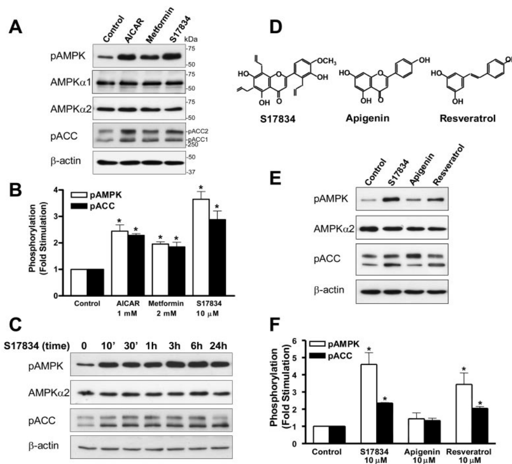
FIG. 1. Polyphenols increase phosphorylation of both AMPK and ACC in cultured human HepG2 hepatocytes. A and B : S17834 (10 \mu M) mimics the effect of AICAR (1 mmol/l) and metformin (2 mmol/l) on AMPK and ACC phosphorylation. HepG2 cells were quiesced in serum-free DMEM overnight and treated with AICAR, metformin, or S17834 for an additional 1 h. Cell lysates (50 \mu g proteins) were resolved by 8% SDS-PAGE as described under RESEARCH DESIGN AND METHODS. The phosphorylation of AMPK and its downstream target, ACC, was assessed by using immunoblots with phospho-Thr-172 AMPK \alpha (pAMPK) and phospho-Ser-79 ACC1 (Ser221 ACC2; pACC) antibodies. The levels of phosphorylated AMPK and the sum of phosphorylated ACC1 and ACC2 were normalized to endogenous AMPK \alpha levels and expressed as the fold stimulation over the basal level (means \pm SE, n = 3 ). C : Time course effect of S17834 on AMPK and ACC phosphorylation. The phosphorylation of AMPK and ACC is shown in HepG2 cells exposed to S17834 (10 \mu M) for 10 and 30 min and 1, 3, 6, and 24 h. D : Chemical structures of polyphenols. E and F : Effect of apigenin and resveratrol on AMPK and ACC phosphorylation. A representative immunoblot and densitometric quantification of the phosphorylation of AMPK and ACC in HepG2 cells incubated with 10 \mu M of polyphenols for 24 h are shown. * P < 0.05 compared with vehicle control.
