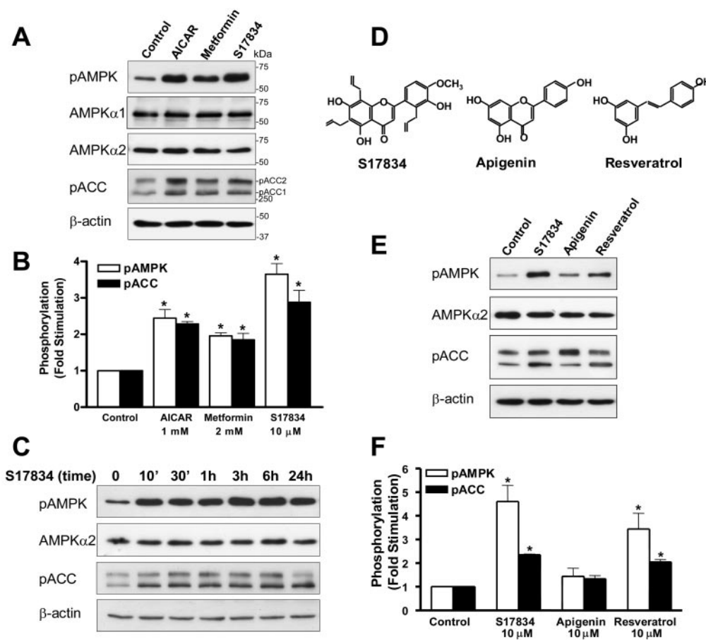
FIG. 1. Polyphenols increase phosphorylation of both AMPK and ACC in cultured human HepG2 hepatocytes. A and B : S17834 (10 \mu M) mimics the effect of AICAR (1 mM) and metformin (2 mM) on AMPK and ACC phosphorylation. HepG2 cells were quiesced in serum-free DMEM overnight and treated with AICAR, metformin, or S17834 for an additional 1 h. Cell lysates (50 \mu g proteins) were resolved by 8% SDS-PAGE as described under RESEARCH DESIGN AND METHODS. The phosphorylation of AMPK and its downstream target, ACC, was assessed by using immunoblots with phospho-Thr-172 AMPK \alpha (pAMPK) and phospho-Ser-79 ACC1 (Ser221 ACC2; pACC) antibodies. The levels of phosphorylated AMPK and the sum of phosphorylated ACC1 and ACC2 were normalized to endogenous AMPK \alpha levels and expressed as the fold stimulation over the basal level (means \pm SE, n = 3 ). C : Time course effect of S17834 on AMPK and ACC phosphorylation. The phosphorylation of AMPK and ACC is shown in HepG2 cells exposed to S17834 (10 \mu M) for 10 and 30 min and 1, 3, 6, and 24 h. D : Chemical structures of polyphenols. E and F : Effect of apigenin and resveratrol on AMPK and ACC phosphorylation. A representative immunoblot and densitometric quantification of the phosphorylation of AMPK and ACC in HepG2 cells incubated with 10 \mu M of polyphenols for 24 h are shown. * P < 0.05 compared with vehicle control.
