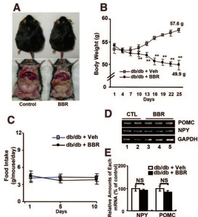
FIG. 1. Effects of berberine on body weight and food intake. A: Gross appearance of whole body and abdomen of vehicle (DMSO, Control, left)-treated or berberine (BBR, right; 5 mg · kg -1 · day -1 )-treated db/db mice. B: Changes of body weight with or without berberine. db/db mice were treated with vehicle (□; n = 16) or berberine (●; n = 17) for 26 days. ** P < 0.001. C: Effects of berberine on food intake. db/db mice were treated with vehicle (□) or berberine (●). D: Quantitative RT-PCR analyses of NPY and POMC genes in the presence or absence of berberine from whole brain. E: Relative amounts of each mRNA were normalized with amounts of glyceraldehyde-3-phosphate dehydrogenase (GAPDH) mRNA and are indicated as fold changes. NS, not significant.
