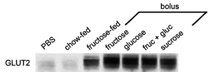
FIG. 3. Dietary regulation of apical GLUT2. Wild-type mice were maintained on 50% complex sugar diet (“chow-fed”) or fructose-rich (65%) diet (“fructose-fed”). Some fructose-fed mice were fasted overnight before they received a gastric bolus of either PBS, glucose, fructose, glucose + fructose, or sucrose (“bolus”). Apical GLUT2 was very low in chow-fed or in fasted animals receiving a PBS bolus. The presence of GLUT2 was high in the apical membrane of animals fed ad libitum with the fructose-rich diet and in the apical membrane of mice receiving a bolus of simple sugar. Reproduced with permission (ref. 15).
