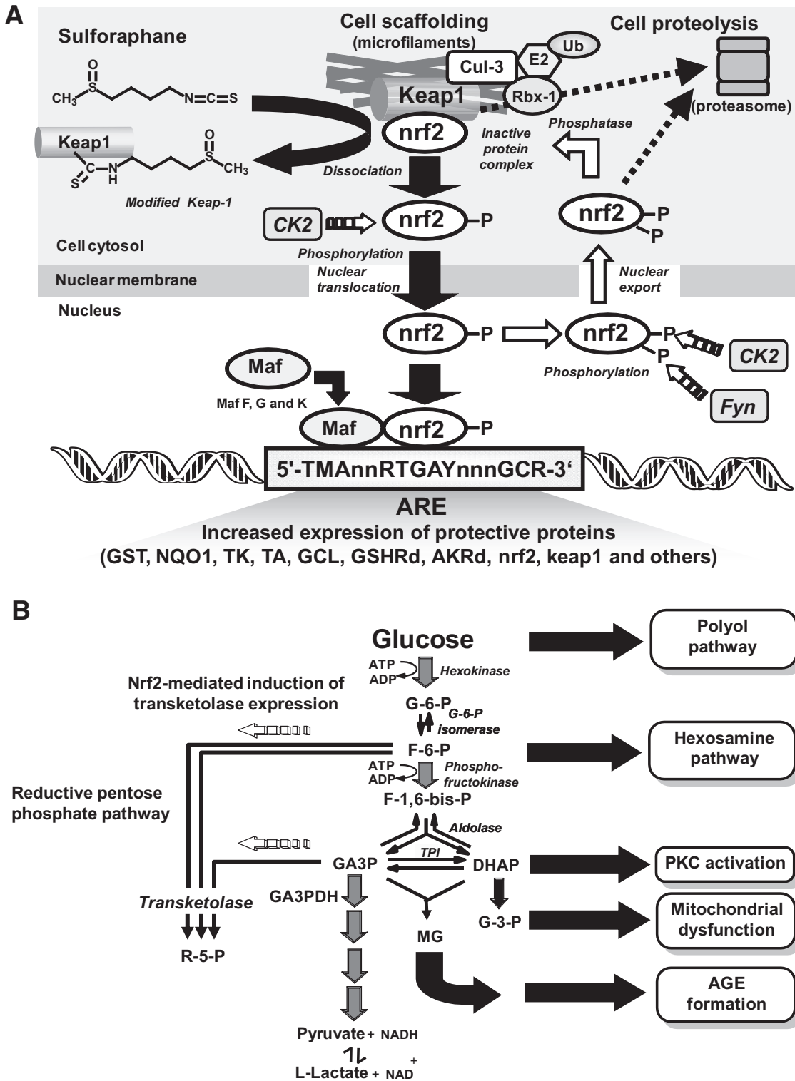
FIG. 1. Nrf2 activation and transketolase expression in human HMEC-1 endothelial cells in vitro. A: Schematic diagram showing activation of nrf2 and dynamic nuclear-cytoplasmic shuttling of nrf2 for ARE-linked expression. B: Multiple pathways of biochemical dysfunction induced by hyperglycemia in microvascular endothelial cells and effect of nrf2 activated, ARE-mediated induction of transketolase expression. Other mechanisms of biochemical dysfunction may be involved.
