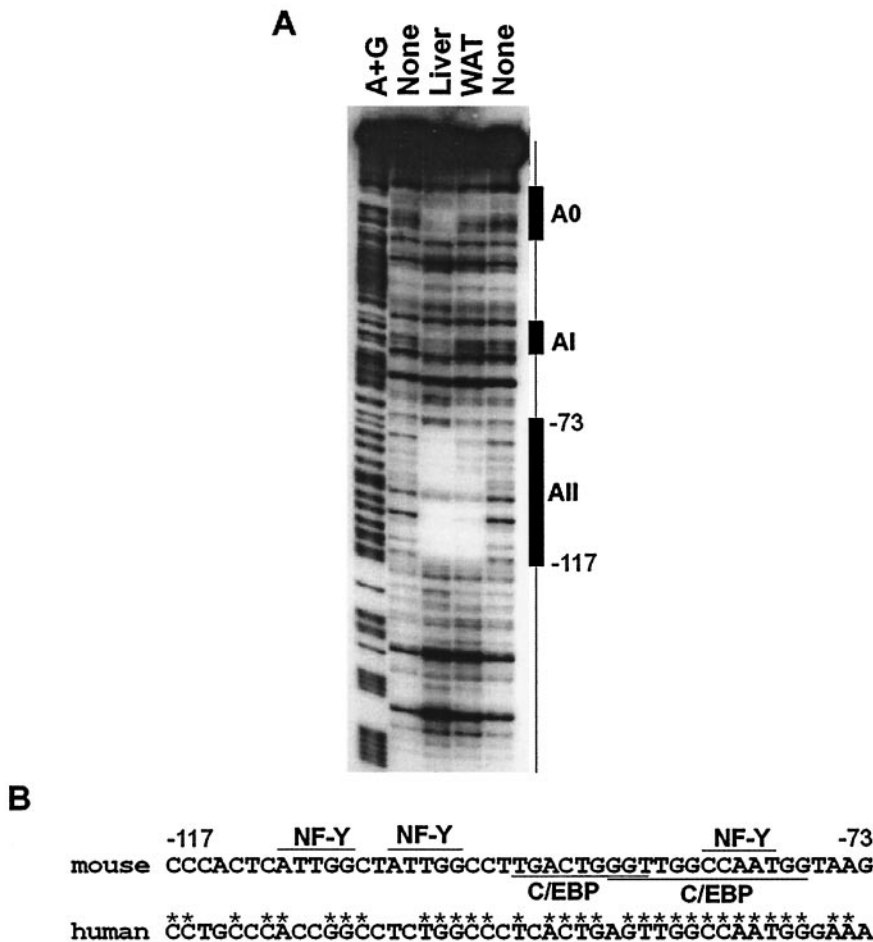
FIG. 2. Nuclear protein binding sites in the mouse adiponectin promoter. A: DNase I footprinting assay of the proximal adiponectin promoter. The mouse adiponectin promoter fragment from -256 to 21 bp was end labeled and used for DNase I footprint analysis with the nuclear extract of rat liver or white adipose tissue (WAT). Three regions (AO, AI, and AII) were protected by liver nuclear extracts, of which only region AII was protected by nuclear extract of white adipose tissue. B: Sequence analysis of region AII ( -117/-73 ). One CCAAT box and two inverted Y-boxes are marked. Two possible C/EBP binding sites were indicated. For comparison, human DNA sequence of the same region was presented, and identical sequences were marked by *.
