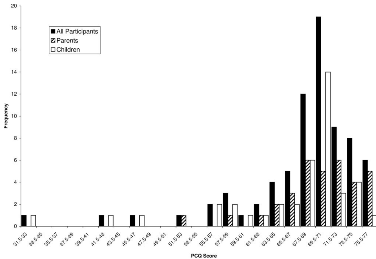
Figure 1 —PCQ score histogram.
