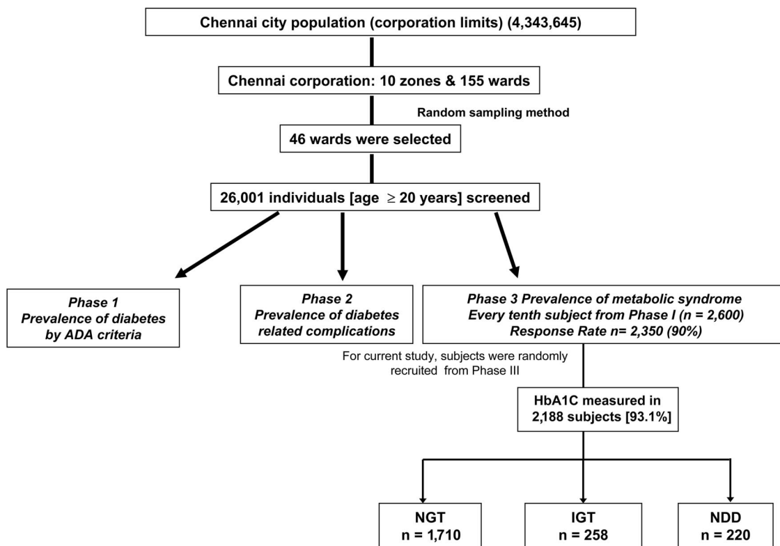
Figure 1 —CURES methodology.
