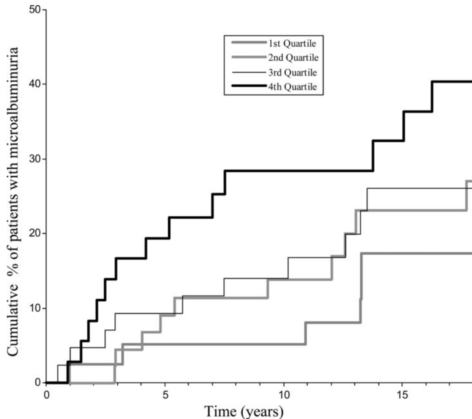
Figure 2 —Kaplan-Meier plot: elevated baseline u-LFABP levels in 165 normoalbuminuric type 1 diabetic patients predict progression to microalbuminuria. Quartiles with limits: u-LFABP/creatinine: 4.7, 10.9 and 21.3 (pg/ml)/(mg/dl). P = 0.02 for overall difference.
