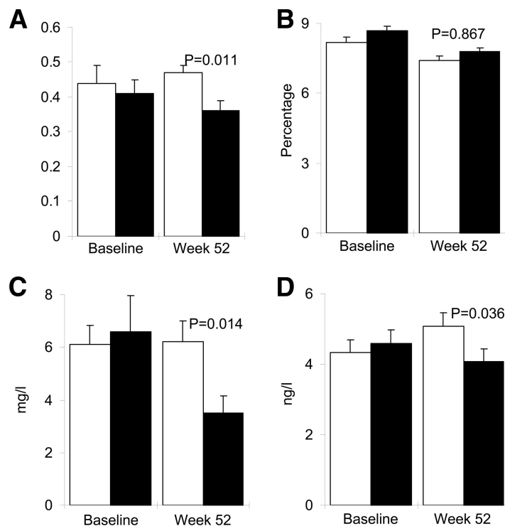
Figure 2 —Change in glycemic and inflammatory markers at study end. Data for PI/I ratio (A), A1C (B), C-reactive protein (C), and IL-6 (D) at baseline and end of study (week 52) in patients treated with anakinra (■) or placebo (□) from baseline until week 13. Data are means \pm SEM.
