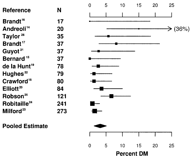
Figure 1—Incidence of diabetes (DM) during acute D+HUS in 13 cohort studies. Point estimates for each study are presented with 95% CIs. The size of each square is proportional to the number of patients in each study. The random-effects pooled estimate was 3.2% (95% CI 1.3–5.1) (see text).
