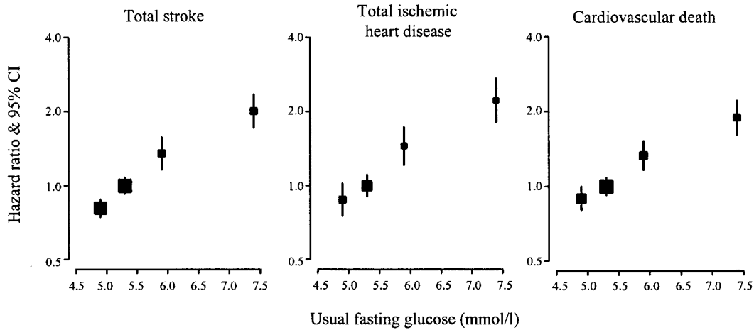
Figure 1 —Usual fasting glucose and risk of cardiovascular end points. The hazard ratios for total (fatal and nonfatal) stroke and IHD and cardiovascular death events adjusted for age, sex, and cohort are plotted on a log scale against usual fasting glucose for each of the four groups defined by baseline fasting glucose (<5, 5–5.9, 6–6.9, \geq 7 mmol/l). The x-axis coordinate for each group is the mean follow-up usual fasting glucose (not the mean baseline fasting glucose [see RESEARCH DESIGN AND METHODS]). For studies without follow-up measurements, weighted average x-axis values were calculated from other cohorts. The 95% CIs for the y-axis coordinate (hazard ratios) are calculated as floating variances, with the glucose group 5–5.9 mmol/l as the reference. The solid squares are larger where there are more events because their size is proportional to the inverse variance, and the vertical lines represent 95% CIs.
