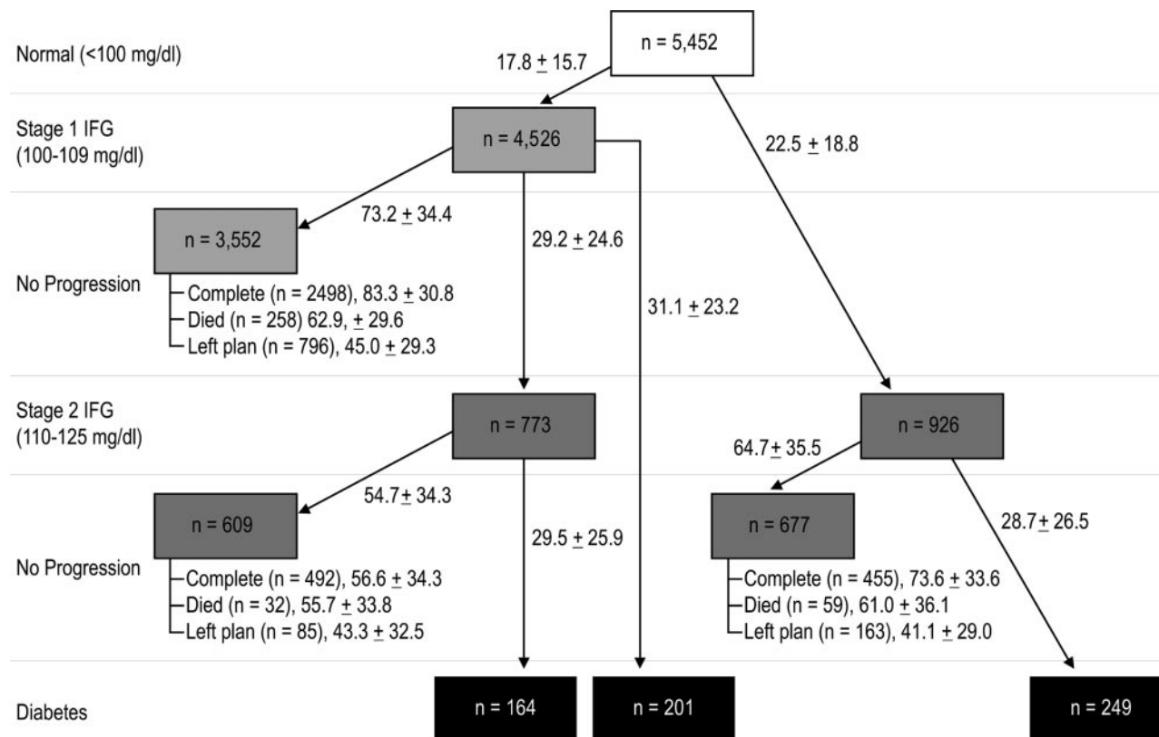
Figure 1 —Progression from normal fasting glucose to stages of IFG to type 2 diabetes. Mean \pm SD months from stage to stage for those who progressed are displayed along each arrow. For those who did not progress, mean \pm SD months of follow-up are displayed along the arrows.
