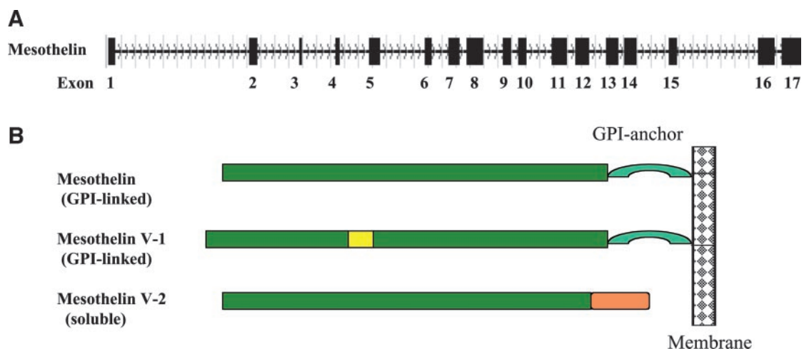
Fig. 2 Schematics describing the mesothelin gene and the proteins it encodes. A , genomic organization of mesothelin gene. There are 17 exons (filled boxes) in the mesothelin gene. B , drawing of three different forms of mesothelin protein described in the database. Mesothelin is the most common variant and is predicted to be membrane-bound; mesothelin V-1 has an additional 8 amino acids (yellow) and is also predicted to be bound to the membrane. Mesothelin V-2 has a modified COOH terminus (orange), lacks the glycosylphosphatidylinositol anchor signal sequence, and is predicted to be secreted.
