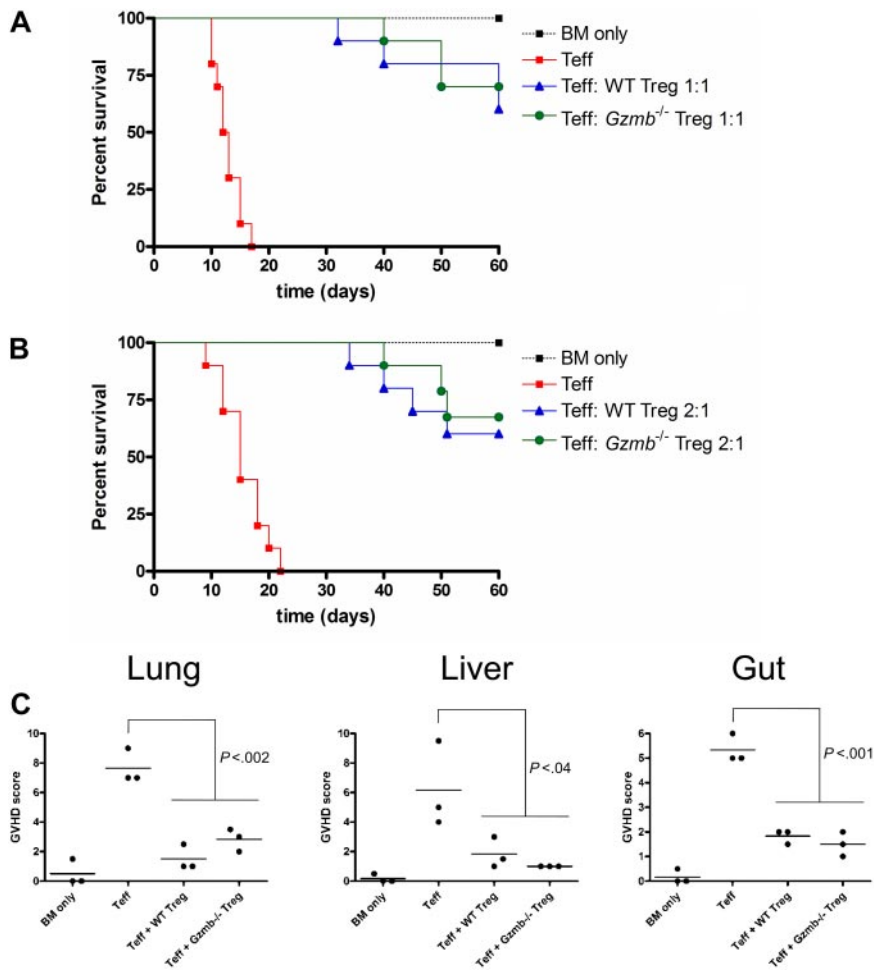
Figure 5. T reg cells do not require granzyme B to rescue hosts from GVHD lethality or to prevent GVHD target organ damage. Lethally irradiated (900 cGy) Balb/c mice received 2 \times 10^5 129/SvJ TCD BM cells with or without 4 \times 10^5 129/SvJ CD25 - T eff cells (both CD4 + and CD8 + ) and either (A) 4 \times 10^5 or (B) 2 \times 10^5 wild-type or Gzmb -/- CD4 + CD25 + T reg cells. Kaplan-Meier survival curves of recipient mice, pooled from 2 independent experiments (n = 10 mice per group), are shown. (C) Seven days after transplantation, 3 mice per experimental group (as outlined in panel A) were killed, and portions of lung, liver, and gut were prepared for histopathologic analysis. There was no statistically significant difference between groups receiving WT or Gzmb -/- T reg cells.
