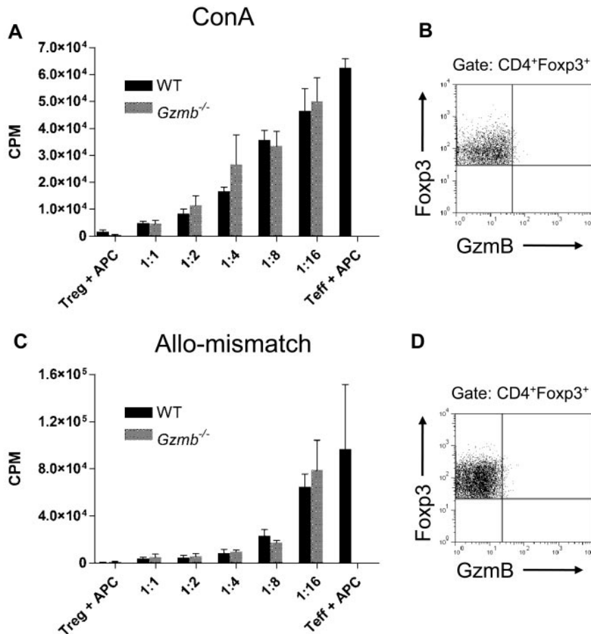
Figure 3. Granzyme B is not required for T_{reg} cell-mediated suppression of ConA-activated and alloactivated T_{eff} -cell proliferation in vitro. (A) Suppression of CD4^+CD25^-T_{eff} -cell proliferation stimulated by ConA in the presence of syngeneic T cell-depleted, irradiated APCs. (B) Representative flow plot of granzyme B expression, gated on wild-type T_{reg} cells cultured for 3 days with ConA-activated T_{eff} cells under maximal suppression conditions (1:1). (C) Dose-dependent suppression of 129/SvJ CD4^+CD25^-T_{eff} -cell proliferation stimulated by fully mismatched Balb/c T cell-depleted APCs. (D) Representative flow plot of granzyme B expression, gated on wild-type T_{reg} cells cultured for 5 days with alloactivated T_{eff} cells under maximal suppression conditions (1:1). All data shown are representative of 3 independent experiments.
