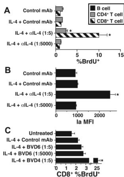
FIGURE 4. In vivo agonist effects of IL-4/blocking anti-IL-4 mAb complex require complex dissociation. A and B , BALB/c mice (four per group) were injected i.p. with IL-4/BVD4-1D11 anti-IL-4 ( \alpha IL-4) complexes or IL-4/control mAb complexes that contained 1 \mu g of IL-4 and 5 or 5000 \mu g of mAb. Mice were injected with BrdU 2 days later and splenocytes were harvested 1 day after that, stained for CD4, CD8, and BrdU ( A ) or CD19, B220, and Ia ( B ) and analyzed by flow cytometry. C , BALB/c mice (four per group) were injected i.p. with IL-4 and complexes of saline, control mAb (5000 \mu g), and BVD6-24G2 anti-IL-4 mAb at low (5 \mu g) or high (5000 \mu g) doses or with BVD4-1D11 anti-IL-4 mAb (5000 \mu g). Mice were injected with BrdU 2 days later and splenocytes were harvested 1 day after that, stained for CD8 and BrdU, and analyzed by flow cytometry. An asterisk (*) indicates a significant increase vs mice that received anything other than IL-4 plus BVD4-1D11 at a 1:5 weight ratio.
