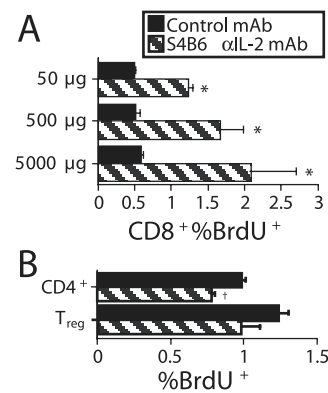
FIGURE 1. S4B6 \alpha IL-2 mAb selectively increases CD8 + T cell proliferation in vivo. BALB/c mice were injected i.p. with the doses of anti-IL-2 ( \alpha IL-2) mAb S4B6 or isotype control mAb (GL117) shown (A) or with 5000 \mu g of these mAbs (B). Two and 2.5 days later, mice were injected i.p. with 600 \mu g of BrdU. Splenocytes were harvested 1 day after that, stained for CD4, CD8, and BrdU (A) or CD4, CD25, Foxp3, and BrdU (B) and analyzed by flow cytometry. An asterisk (*) signifies a significant increase in the percentage of BrdU + cells vs mice treated with the same dose of control mAb; a cross (†) indicates a significant decrease in the percentage of BrdU + cells vs mice treated with the same dose of control mAb.
