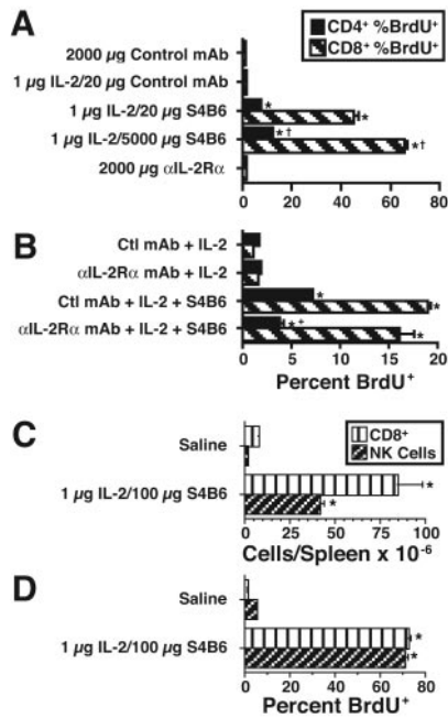
FIGURE 2. IL-2/S4B6 complexes are functionally active and act independently of IL-2R \alpha . A , BALB/c mice were injected with 2,000 \mu g of anti-IL-2R \alpha ( \alpha IL-2R \alpha ) or saline 2 days before and at the time of injection of 1 \mu g of IL-2 plus 20 or 5,000 \mu g of S4B6 or 20 \mu g of isotype control mAb. Mice were injected with BrdU 2 days later. Their spleen cells were stained for CD4, CD8, and BrdU 1 day after that and analyzed by flow cytometry. B , BALB/c mice were injected with 2,000 \mu g of anti-IL-2R \alpha or isotype control mAb 1 day before and at the time of injection of 1 \mu g of IL-2 with or without 5 \mu g of S4B6, and proliferative responses by their spleen cells were evaluated as in A . C and D , In a separate experiment, BALB/c mice were injected with saline or 100 \mu g of S4B6 plus 1 \mu g of IL-2 on days 0 and 2 and with BrdU on day 2, and sacrificed on day 3. Spleen cells were counted, stained for CD3, CD8, CD49b, and BrdU, and analyzed by flow cytometry for the numbers of CD8 ^+ T cells (CD3 ^+ CD8 ^+ ) and NK cells (CD3 ^- CD49b ^+ ) per spleen and for the percentage of these cells that were BrdU ^+ . An asterisk (*) indicates a significant increase in cell number or the percentage of BrdU ^+ cells vs mice treated with the same dose of control mAb; a cross (†) indicates a significant increase in the percentage of BrdU ^+ cells vs mice treated with IL-2 plus 20 \mu g of S4B6; a plus sign (+) indicates a significant decrease in the percentage of BrdU ^+ cells vs mice treated with control mAb instead of anti-IL-2R \alpha mAb.
